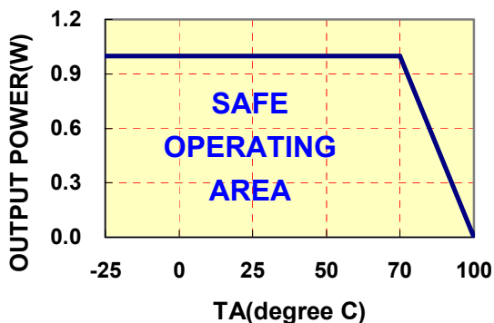
DERATING CURVE
