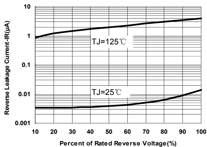
Fig.2-Typical Reverse Characteristics
