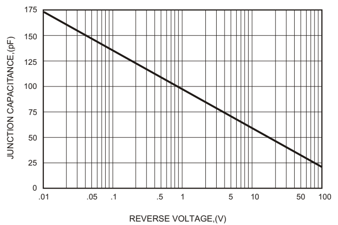
FIG.5-TYPICAL JUNCTION CAPACITANCE
