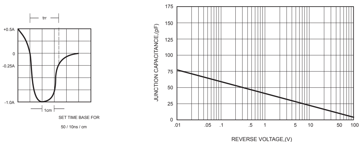
FIG.5-TYPICAL JUNCTION CAPACITANCE
