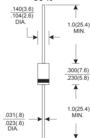
DO-15
