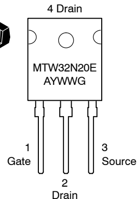
TO-247 CASE 340L STYLE 1
