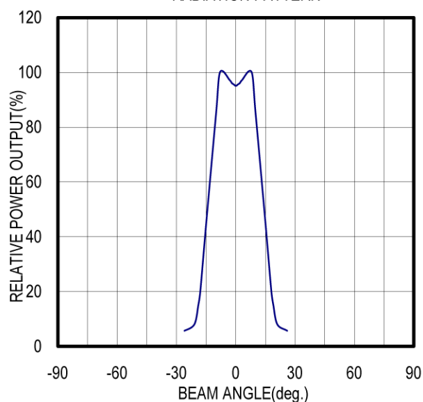
RADIATION PATTERN
