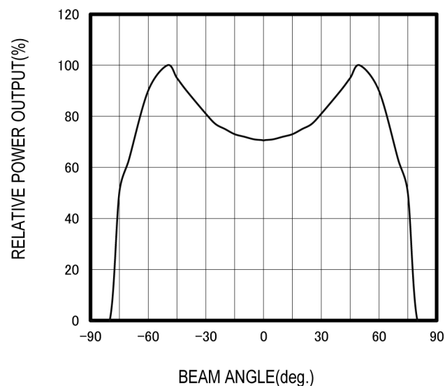
RADIATION PATTERN
