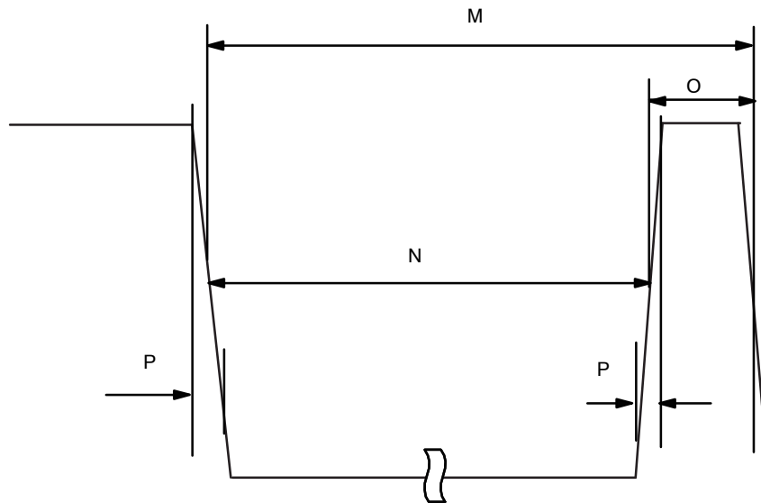
Figure 63. V Pulse
