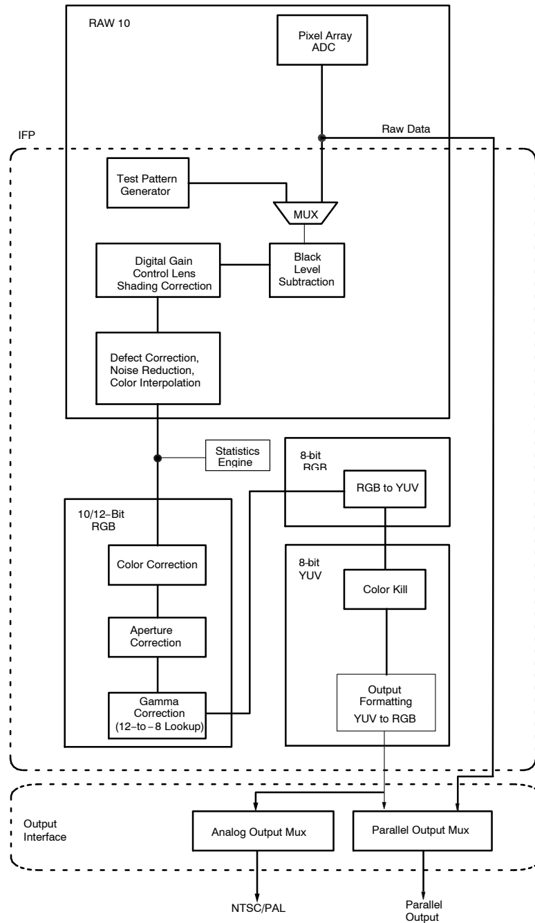
Figure 10. Color Pipeline
