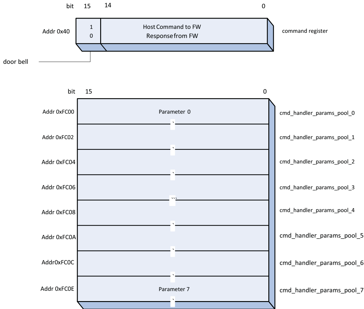
Figure 23. Interface Structure
