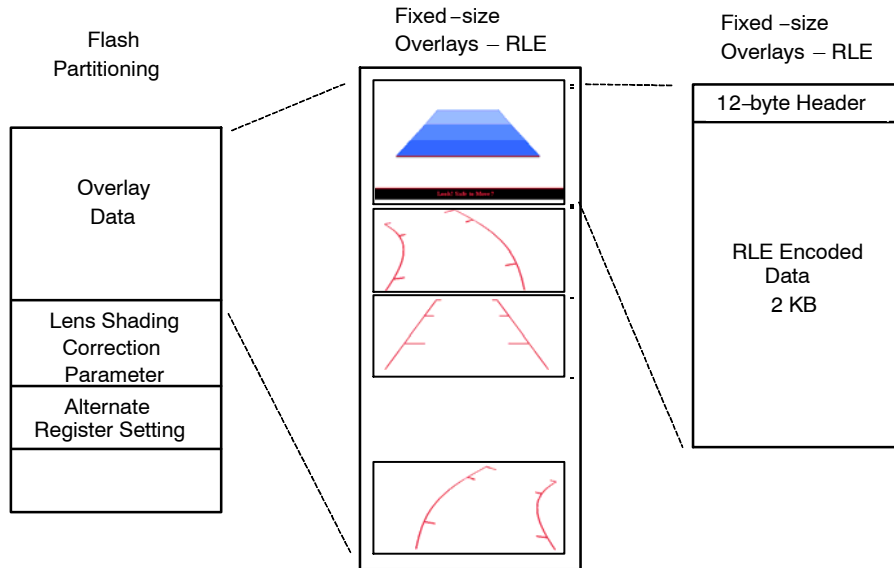
Figure 36. Memory Partitioning
