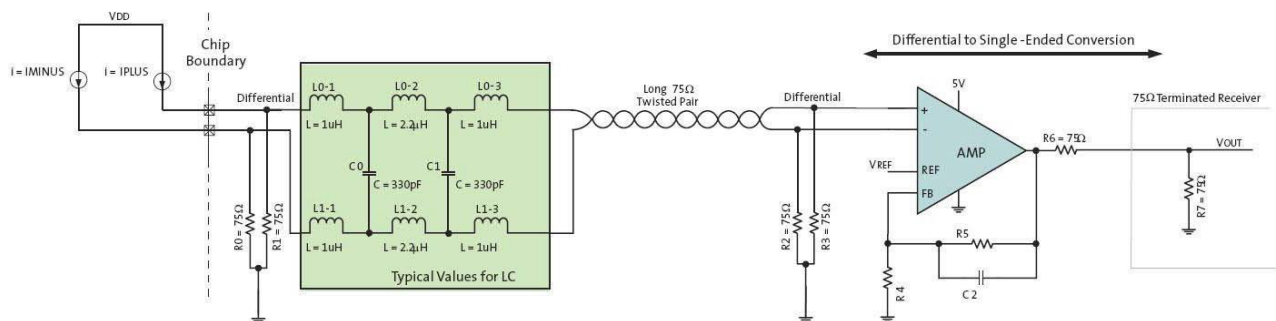
Figure 42. Differential Connection—Grounded Termination
