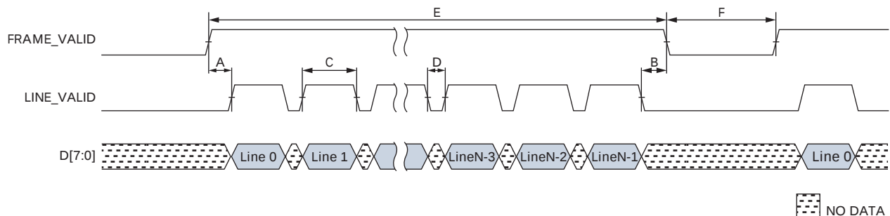
Figure 11: Vertical Timing
