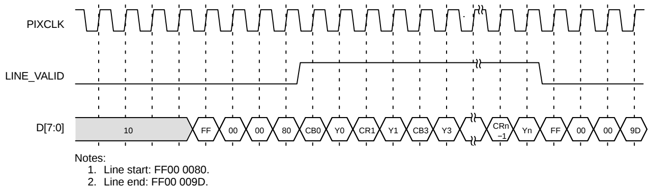
Figure 12. Horizontal Timing
