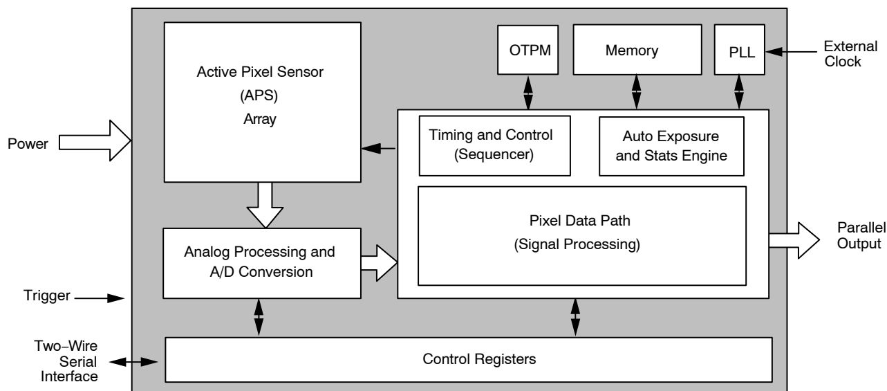
Figure 1. Block Diagram
