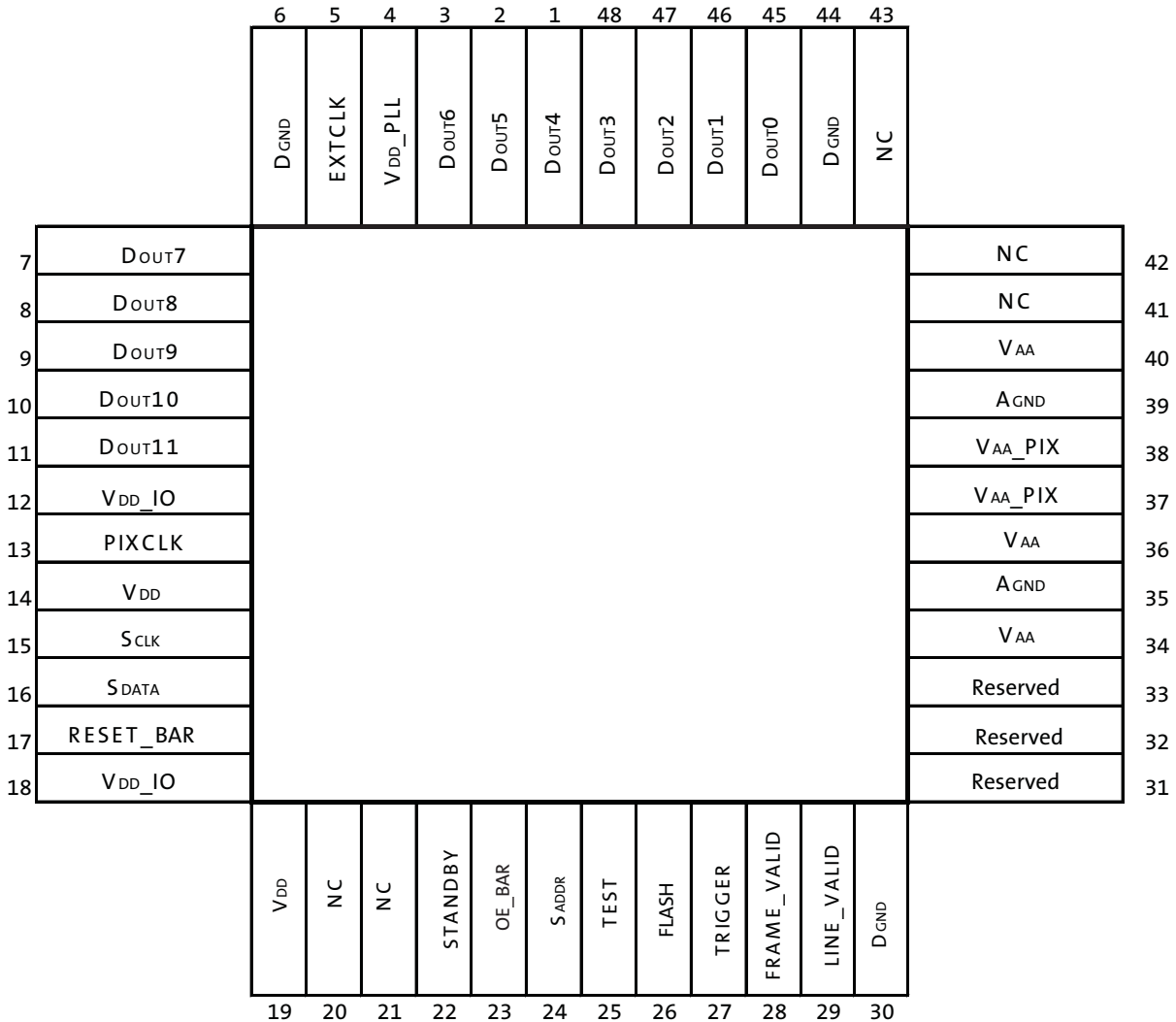
Figure 3: 48 iLCC Package, Parallel Output
