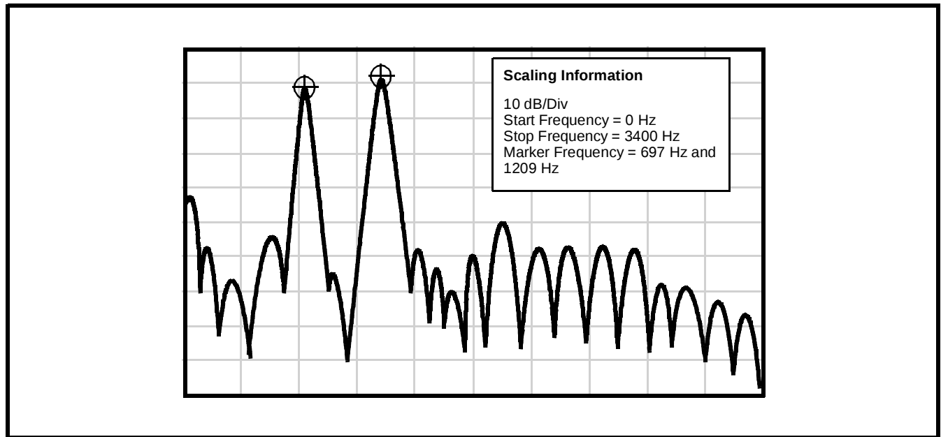
Figure 10 - Spectrum Plot
