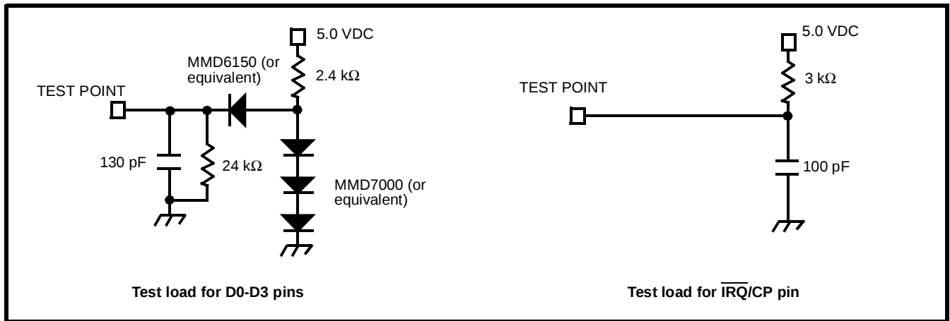
Figure 14 - Test Circuits
