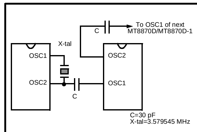
Figure 7 - Oscillator Connection
