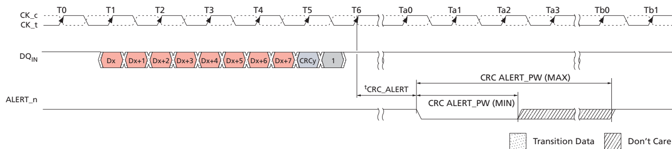
Figure 105: CRC Error Reporting
