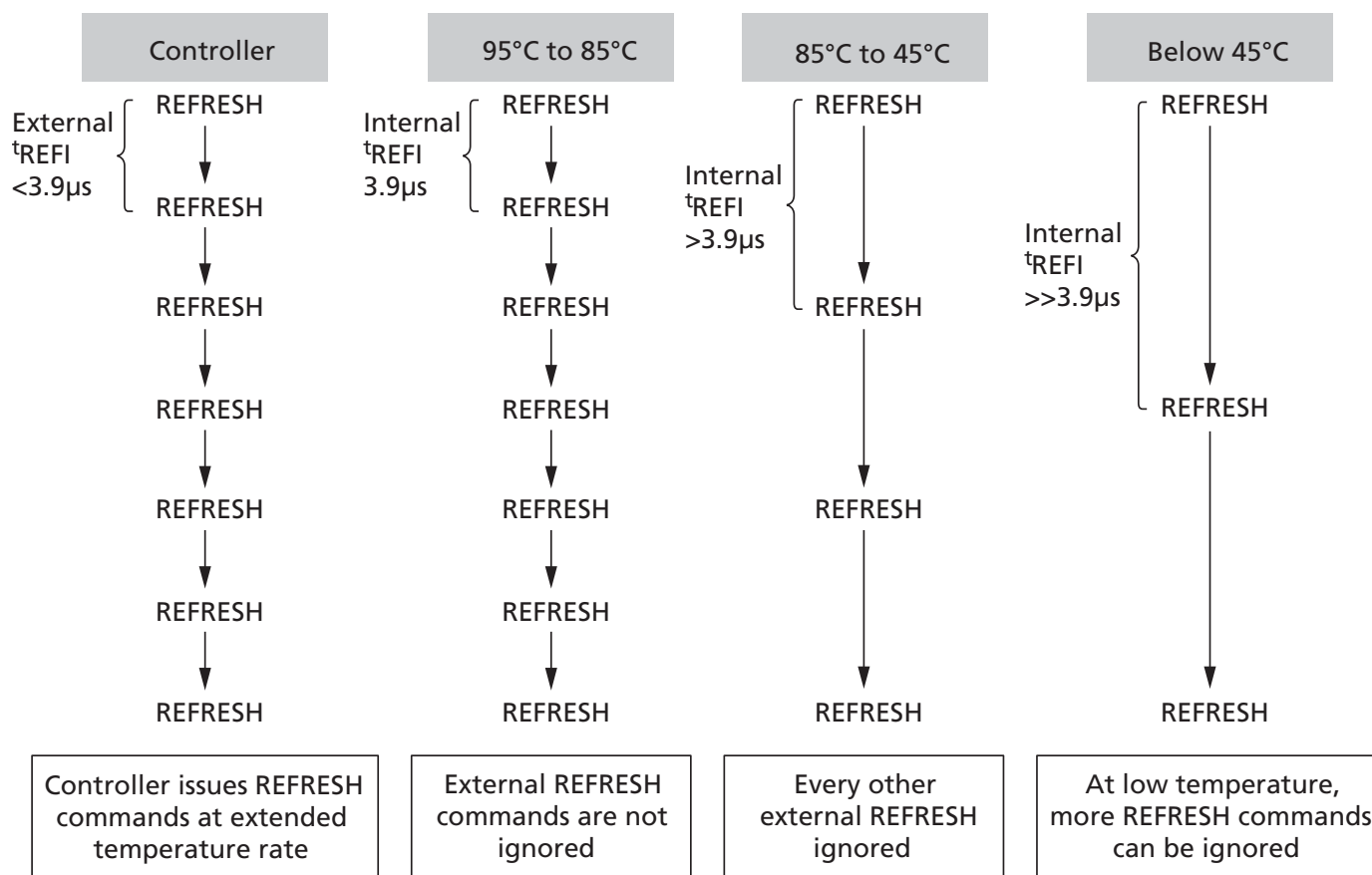
Figure 83: TCR Mode Example 1
