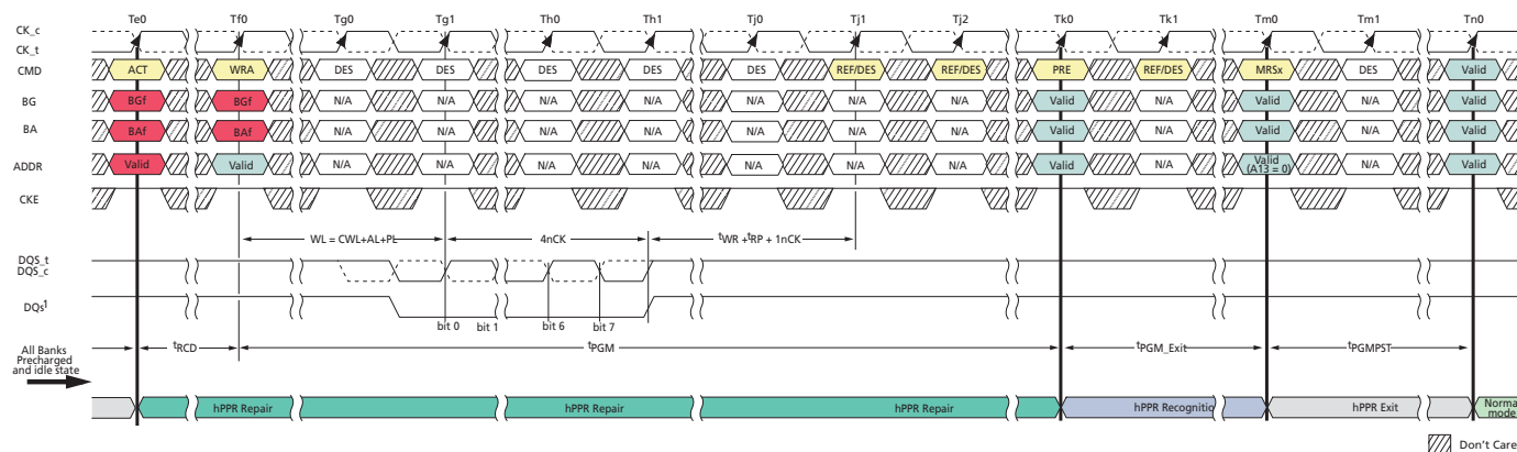
Figure 73: hPPR WRA – Repair and Exit
