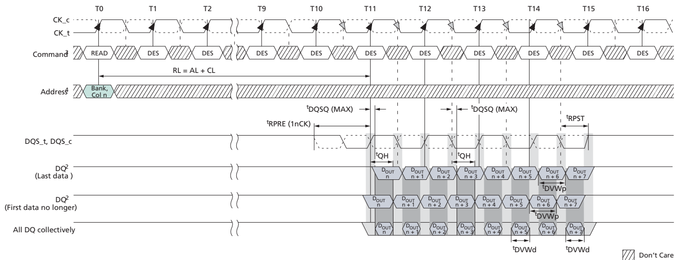
Figure 123: Data Strobe-to-Data Relationship
