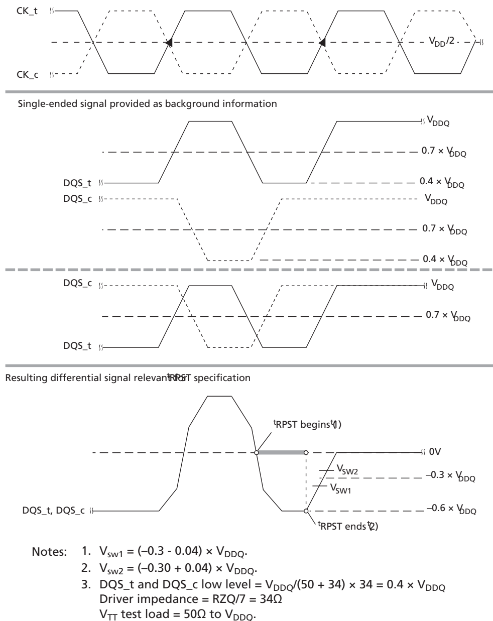
Figure 126: t_{RPST} Method for Calculating Transitions and Endpoints
