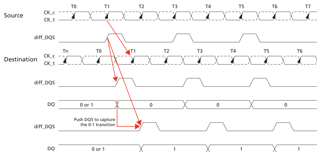
Figure 19: Write Leveling Concept, Example 1
