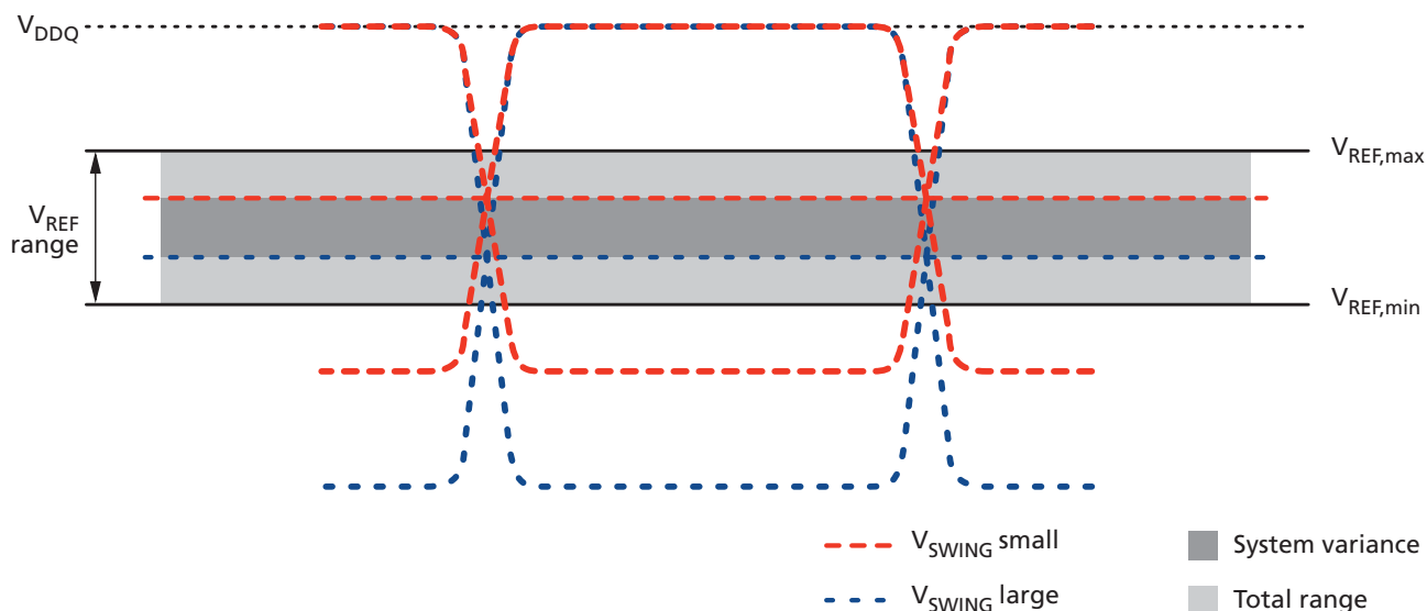
Figure 62: V_{\text{REFDQ}} Voltage Range
