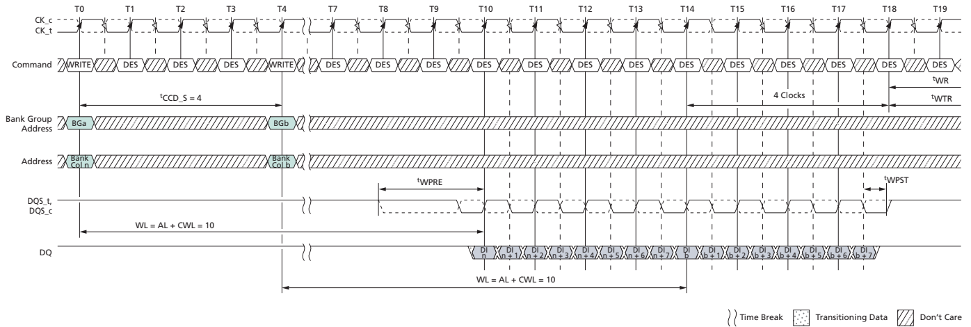
Figure 172: Consecutive WRITE (BL8) with 2^t\text{CK} Preamble in Different Bank Group
