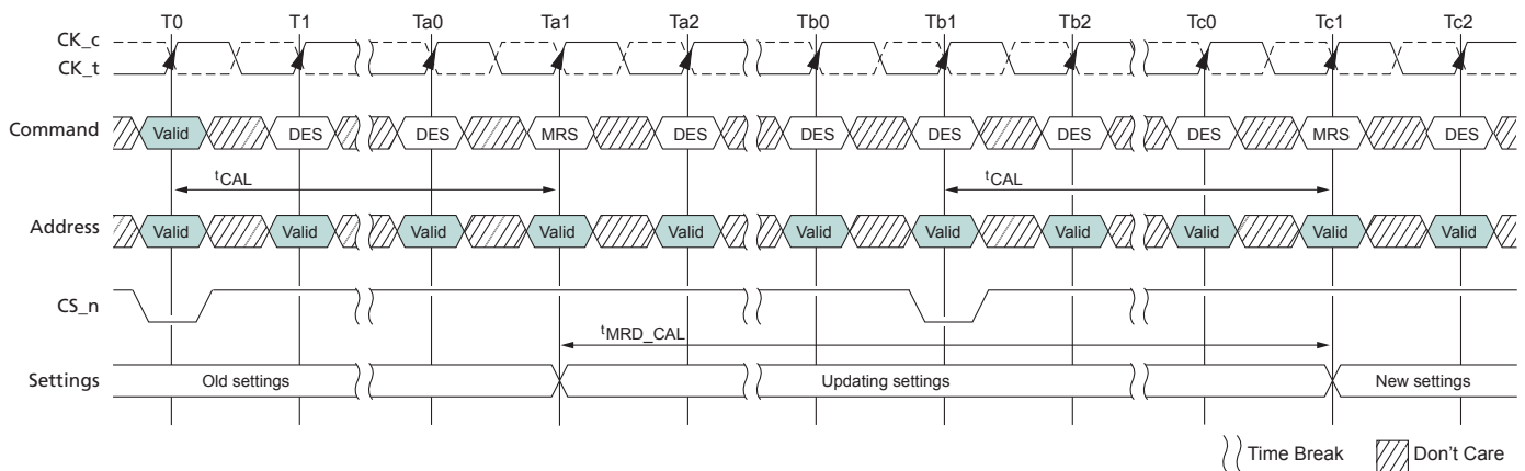
Figure 28: t_{MRD\_CAL} , Mode Register Cycle Time With CAL Enabled
