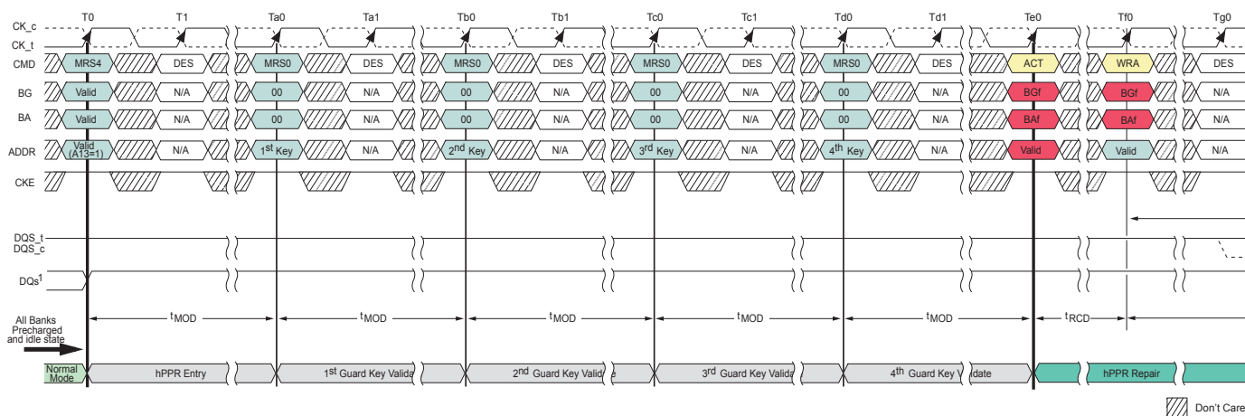
Figure 72: hPPR WRA – Entry
