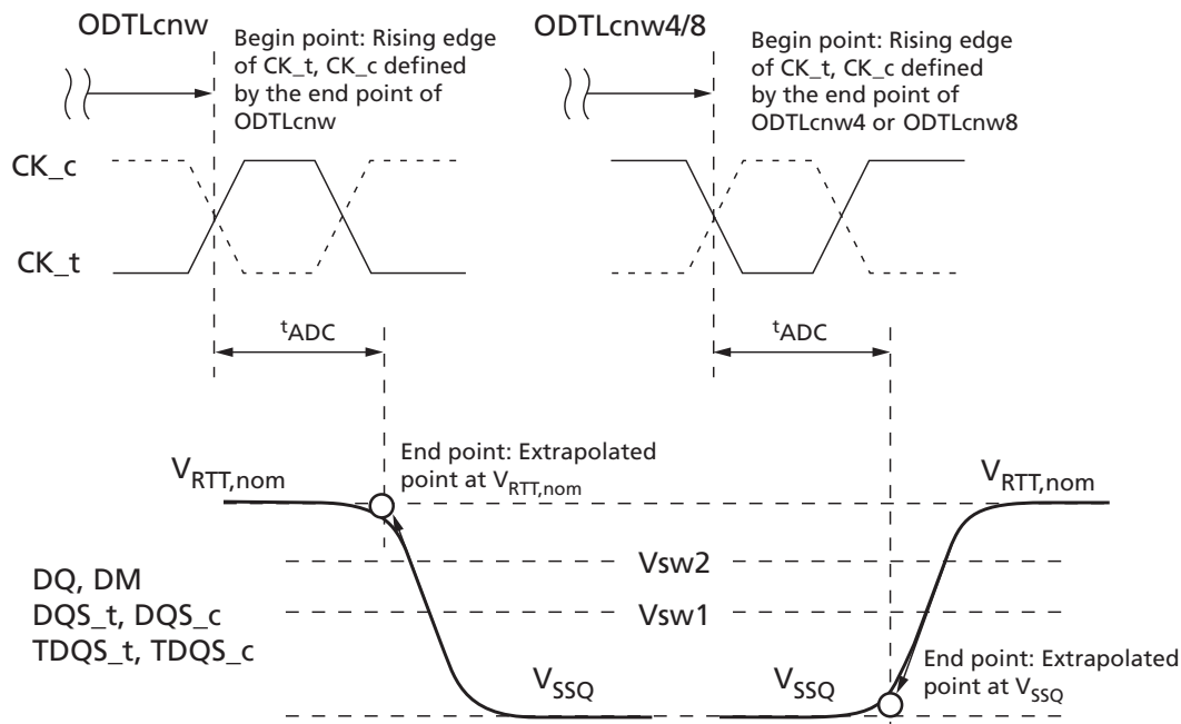
Figure 239: t_{ADC} Definition with Dynamic ODT Control
