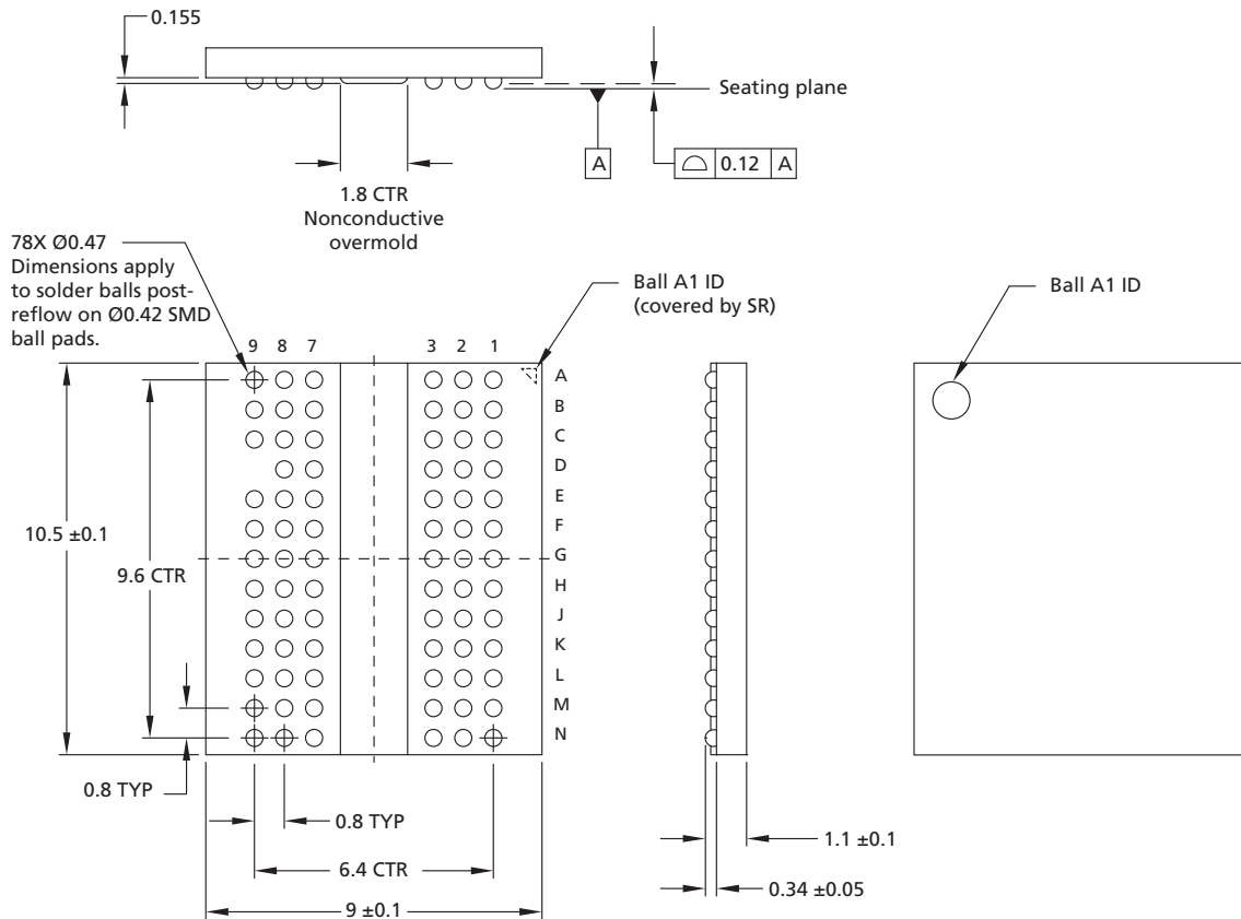
Figure 8: 78-Ball FBGA – x4, x8 "RH"
