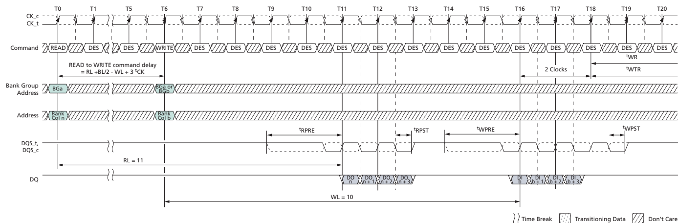
Figure 144: READ (BC4) Fixed to WRITE (BC4) Fixed with 2^t\text{CK} Preamble in Same or Different Bank Group
