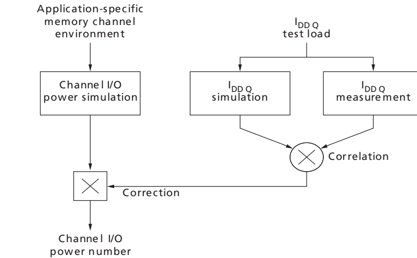
Figure 243: Correlation: Simulated Channel I/O Power to Actual Channel I/O Power
