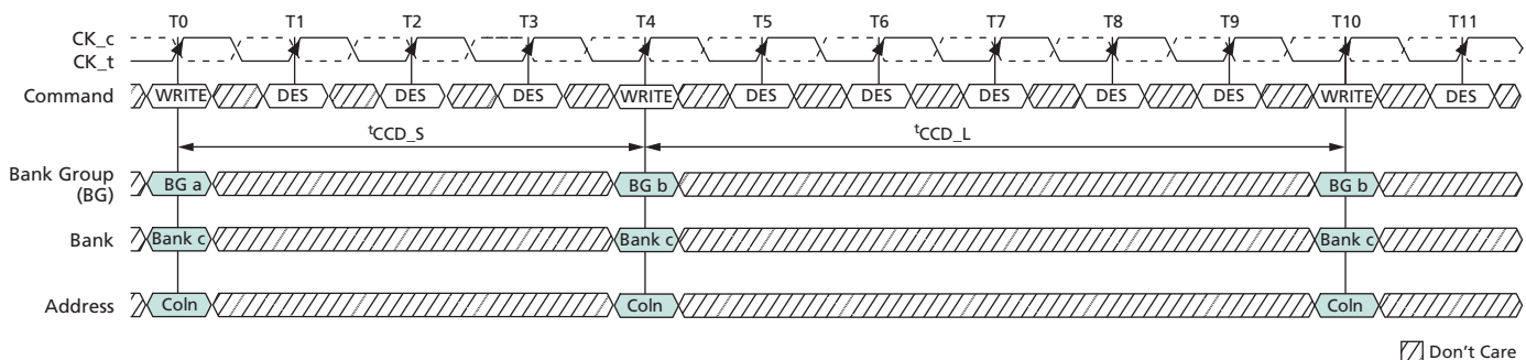
Figure 117: Write Burst t_{CCD\_S} and t_{CCD\_L} Examples
