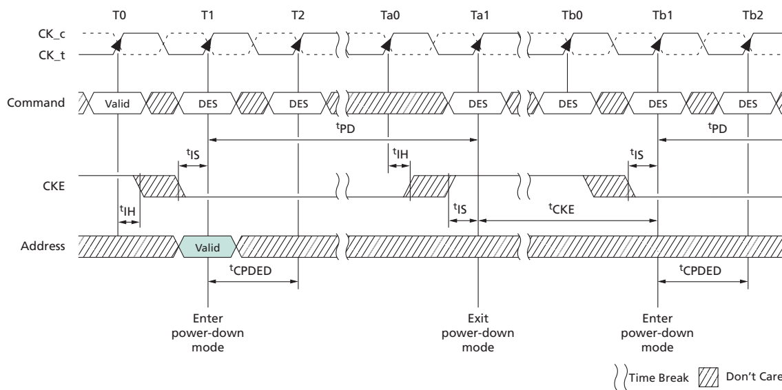
Figure 99: Power-Down Entry/Exit Clarifications – Case 1
