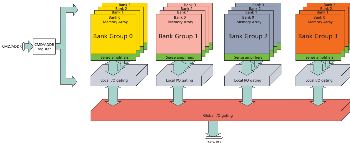
Figure 115: Bank Group x4/x8 Block Diagram
