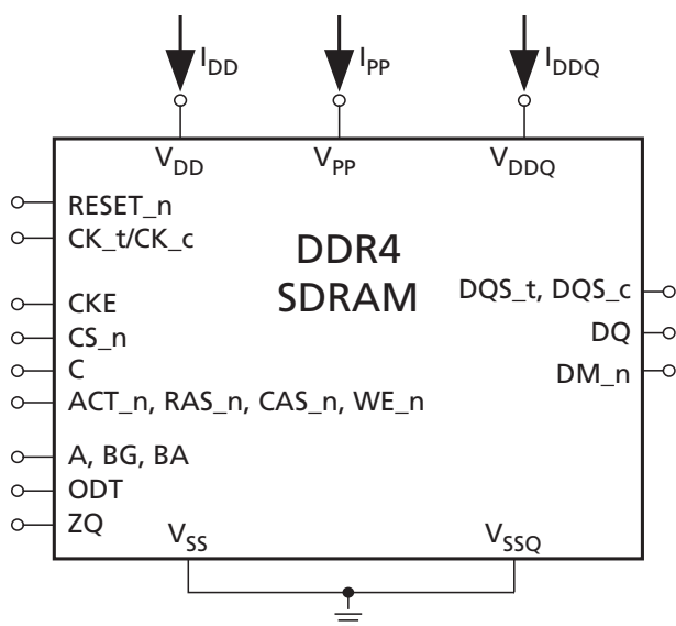
Figure 242: Measurement Setup and Test Load for I_{DDx} , I_{DDPx} , and I_{DDQx}
