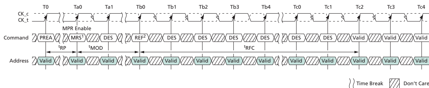
Figure 38: REFRESH Timing
