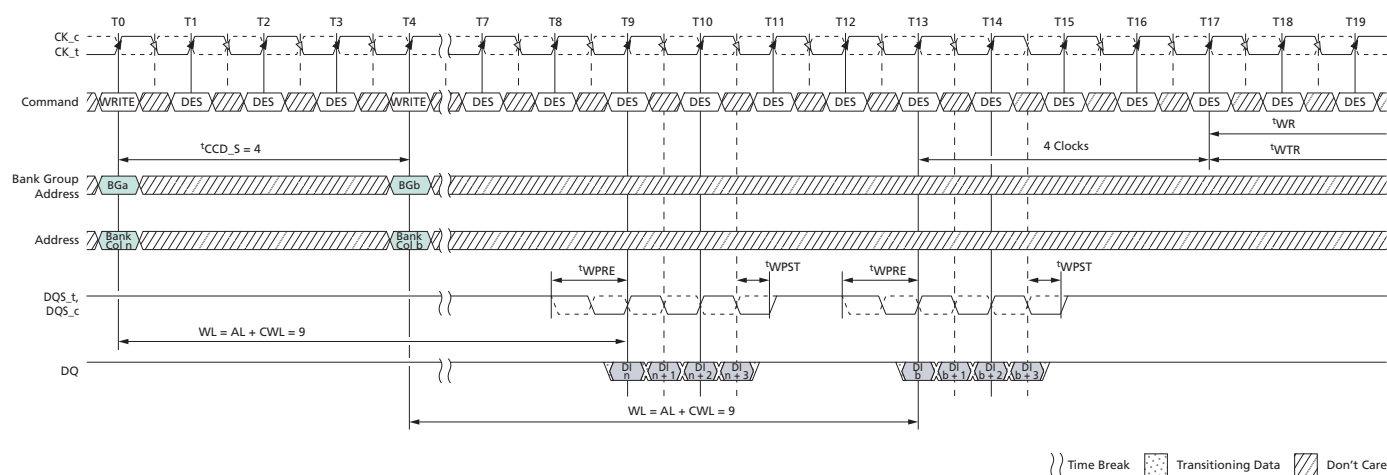
Figure 175: WRITE (BC4) OTF to WRITE (BC4) OTF with 1^tCK Preamble in Different Bank Group
