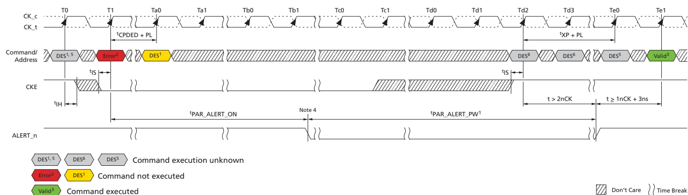
Figure 51: CA Parity Error Checking – SRE Attempt
