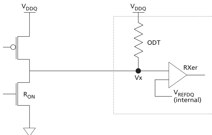
Figure 70: V_{\text{REFDQ}} Equivalent Circuit
