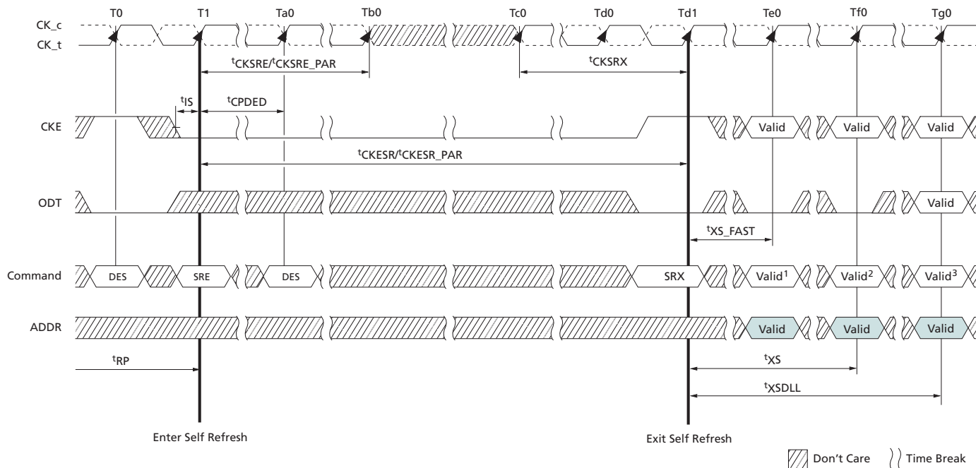
Figure 86: Self Refresh Entry/Exit Timing
