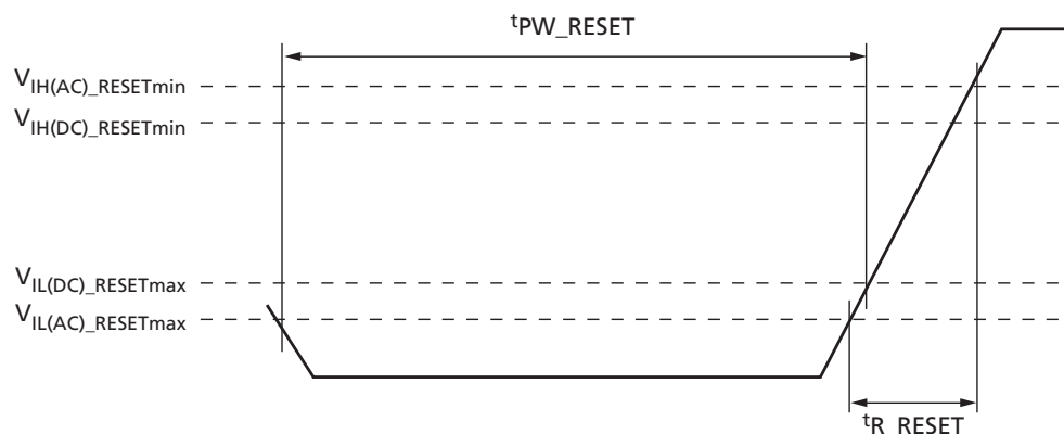
Figure 216: CT Type-D Input Slew Rate Definition
