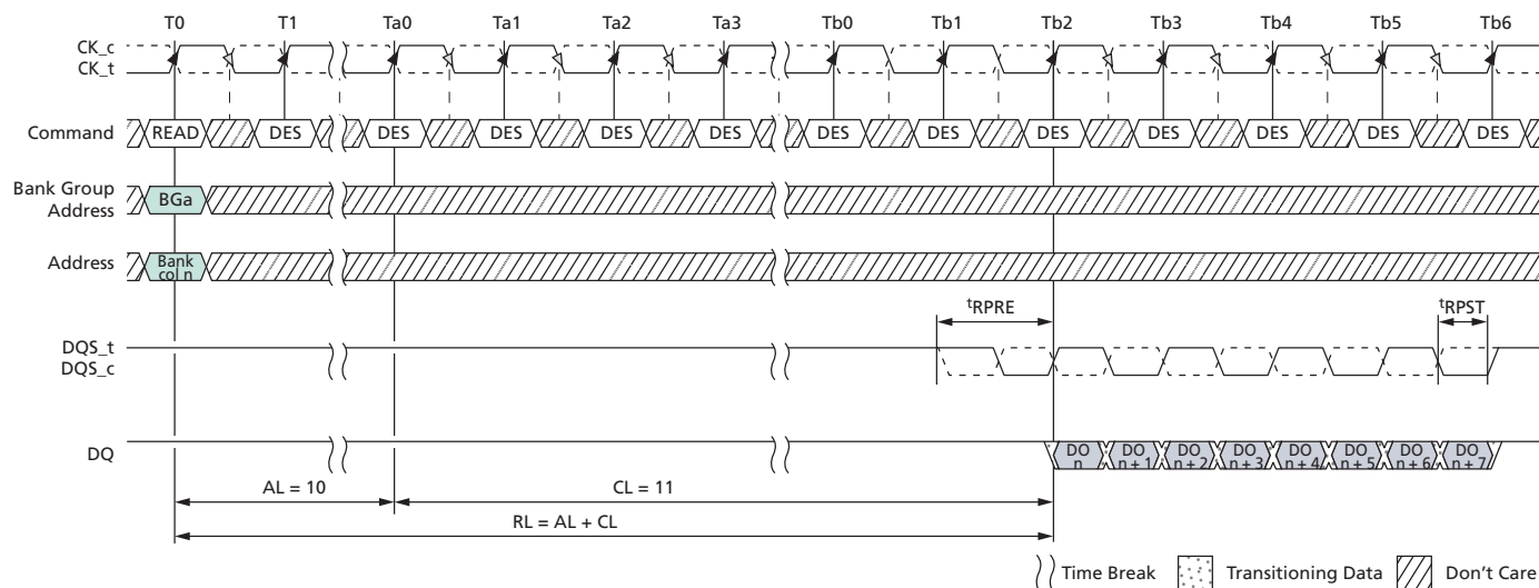
Figure 128: READ Burst Operation, RL = 21 (AL = 10, CL = 11, BL8)
