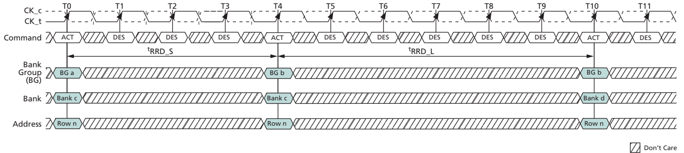
Figure 118: t_{RRD} Timing
