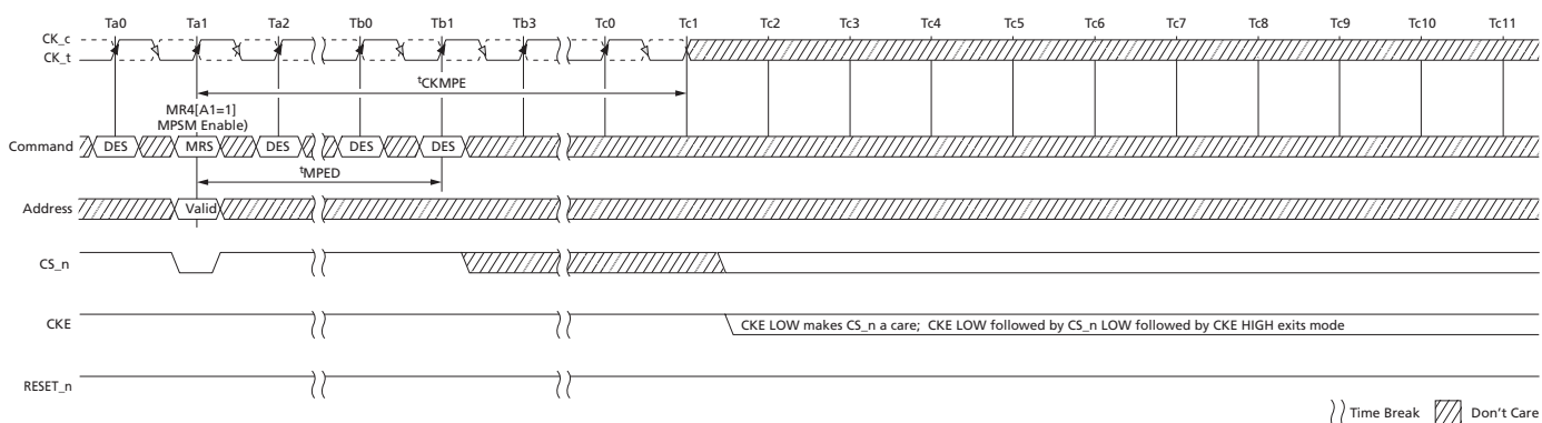
Figure 44: Maximum Power-Saving Mode Entry
