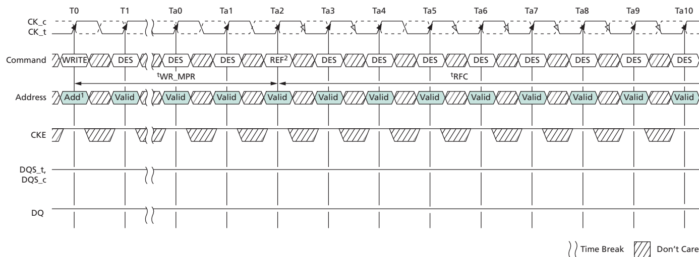
Figure 40: WRITE-to-REFRESH Timing
