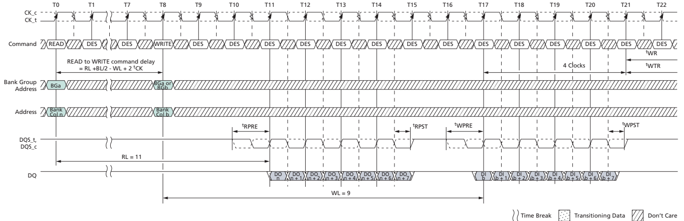
Figure 139: READ (BL8) to WRITE (BL8) with 1 t CK Preamble in Same or Different Bank Group
