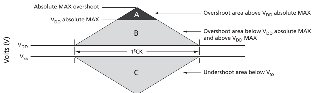
Figure 225: ADDR, CMD, CNTL Overshoot and Undershoot Definition
