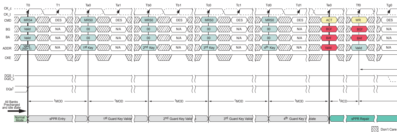
Figure 76: sPPR – Entry
