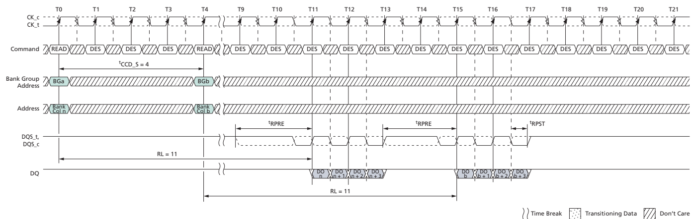
Figure 134: READ (BC4) to READ (BC4) with 2 nd CK Preamble in Different Bank Group
