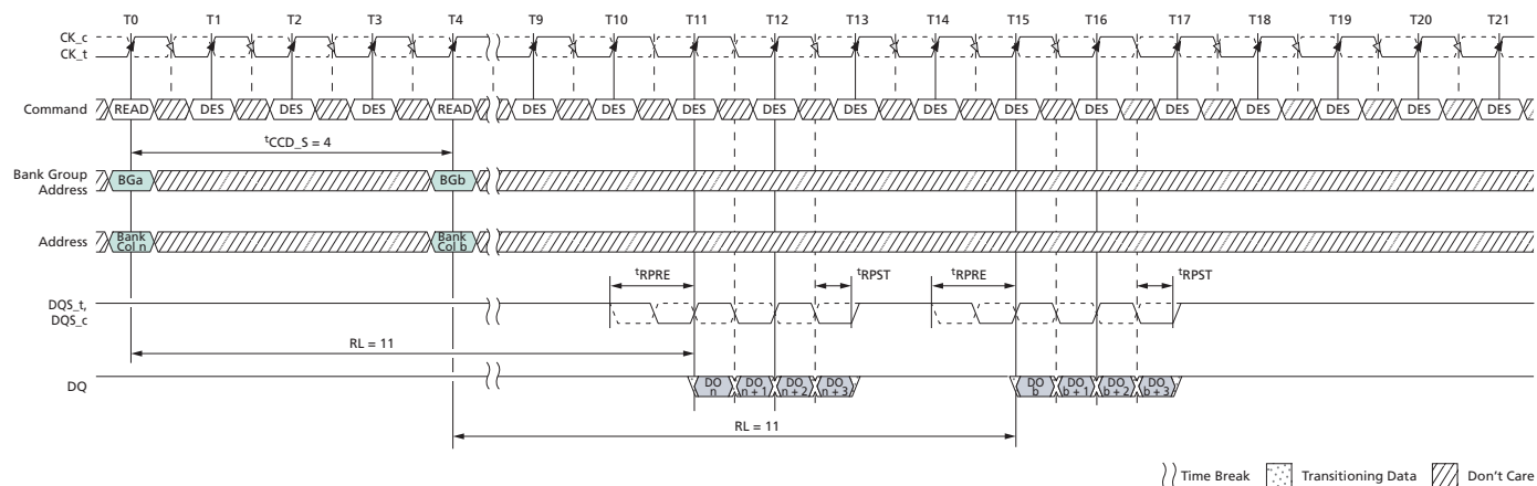
Figure 133: READ (BC4) to READ (BC4) with 1 st CK Preamble in Different Bank Group
