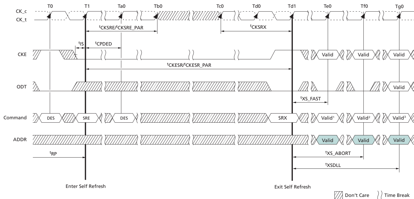
Figure 88: Self Refresh Abort
