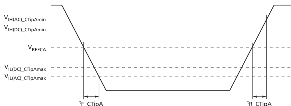
Figure 213: CT Type-A Input Slew Rate Definition
