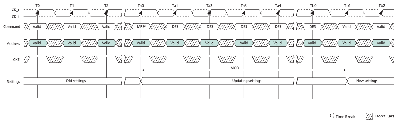
Figure 15: t^{\text{MOD}} Timing
