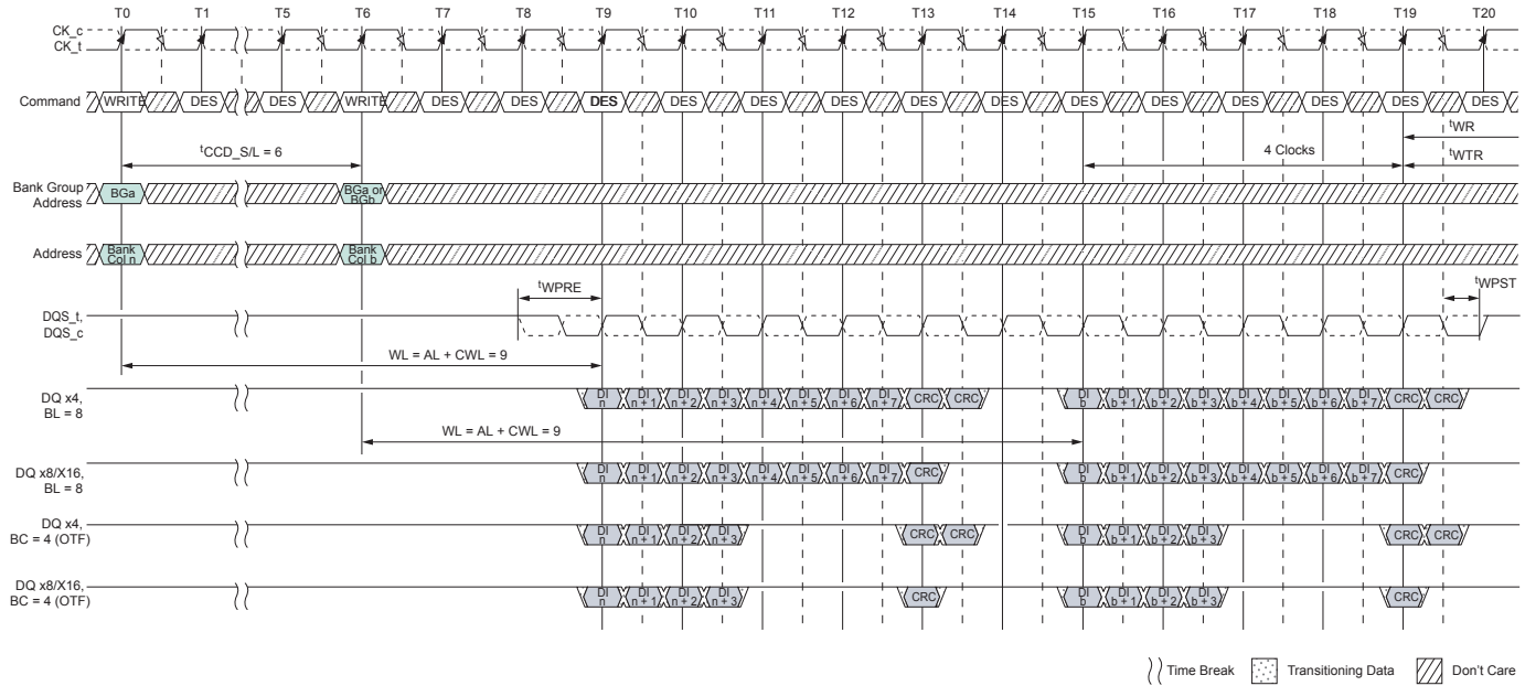
Figure 195: Nonconsecutive WRITE (BL8/BC4-OTF) with 1 t CK Preamble and Write CRC in Same or Different Bank Group
