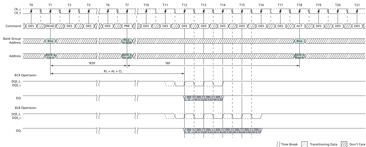
Figure 149: READ to PRECHARGE with 1 t CK Preamble
