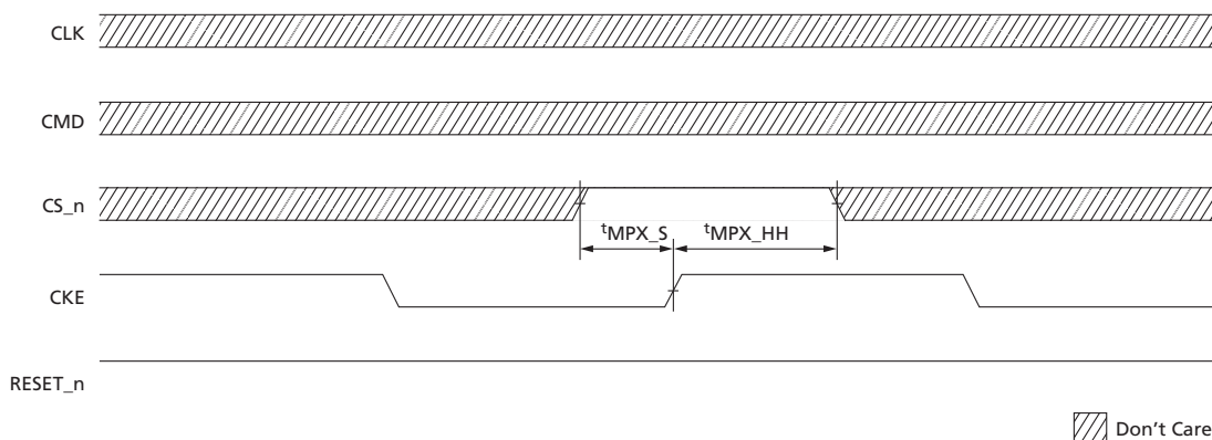
Figure 46: Maintaining Maximum Power-Saving Mode with CKE Transition
