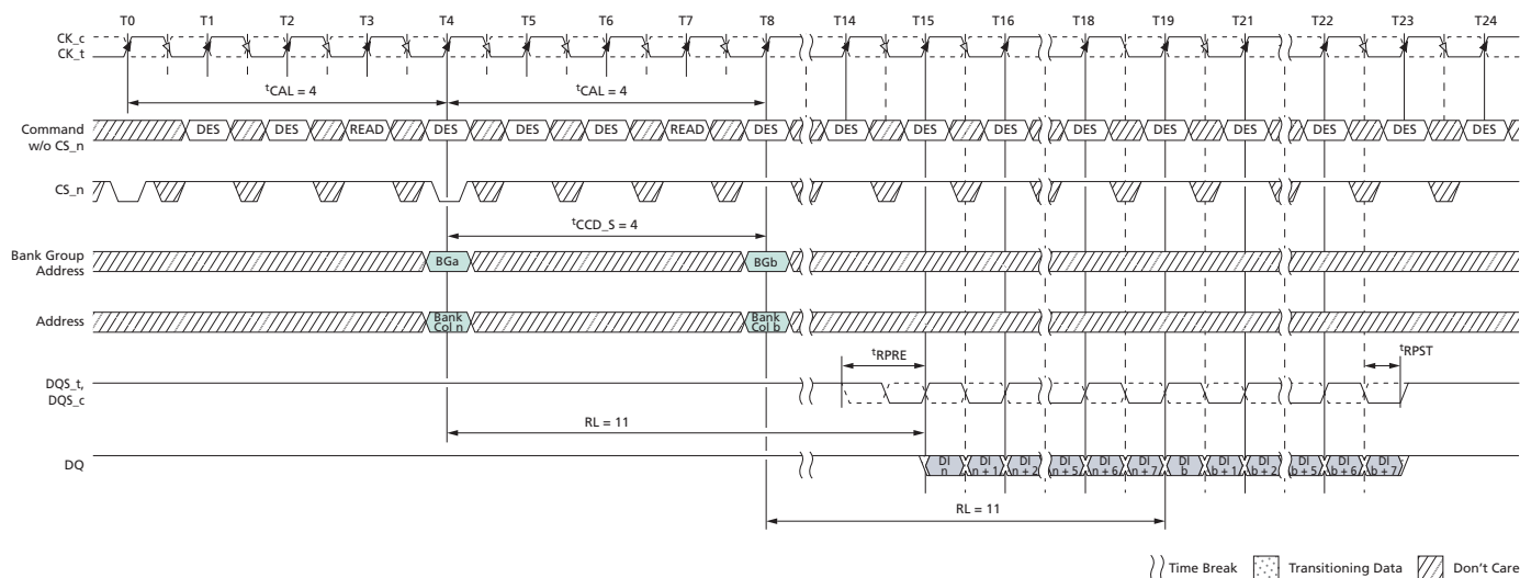
Figure 160: Consecutive READ (BL8) with CAL ( 4^t\text{CK} ) and 1^t\text{CK} Preamble in Different Bank Group
