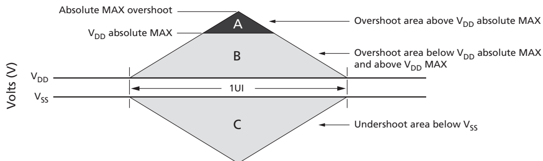
Figure 226: CK Overshoot and Undershoot Definition
