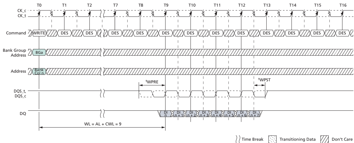
Figure 169: WRITE Burst Operation, WL = 9 (AL = 0, CWL = 9, BL8)
