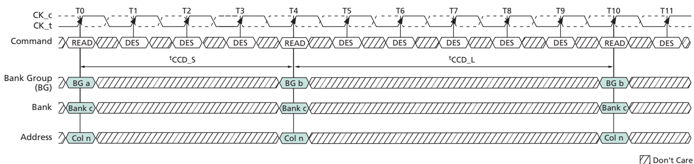
Figure 116: READ Burst t_{CCD\_S} and t_{CCD\_L} Examples
