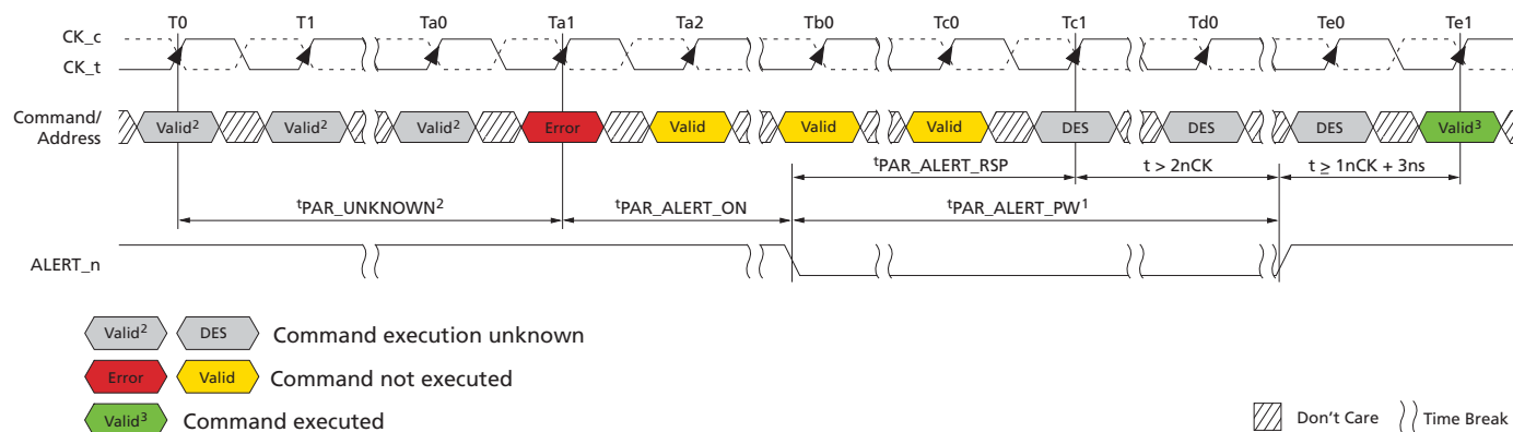
Figure 50: Persistent CA Parity Error Checking Operation
