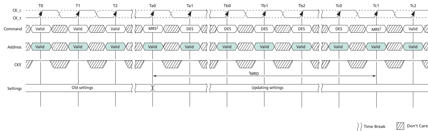
Figure 14: t^{\text{MRD}} Timing
