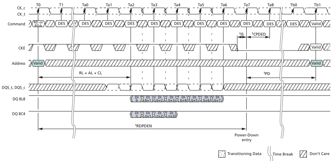
Figure 91: Power-Down Entry After Read and Read with Auto Precharge
