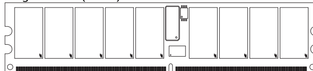
Figure 1: 240-Pin DIMM (MO-237 R/C “K”)
