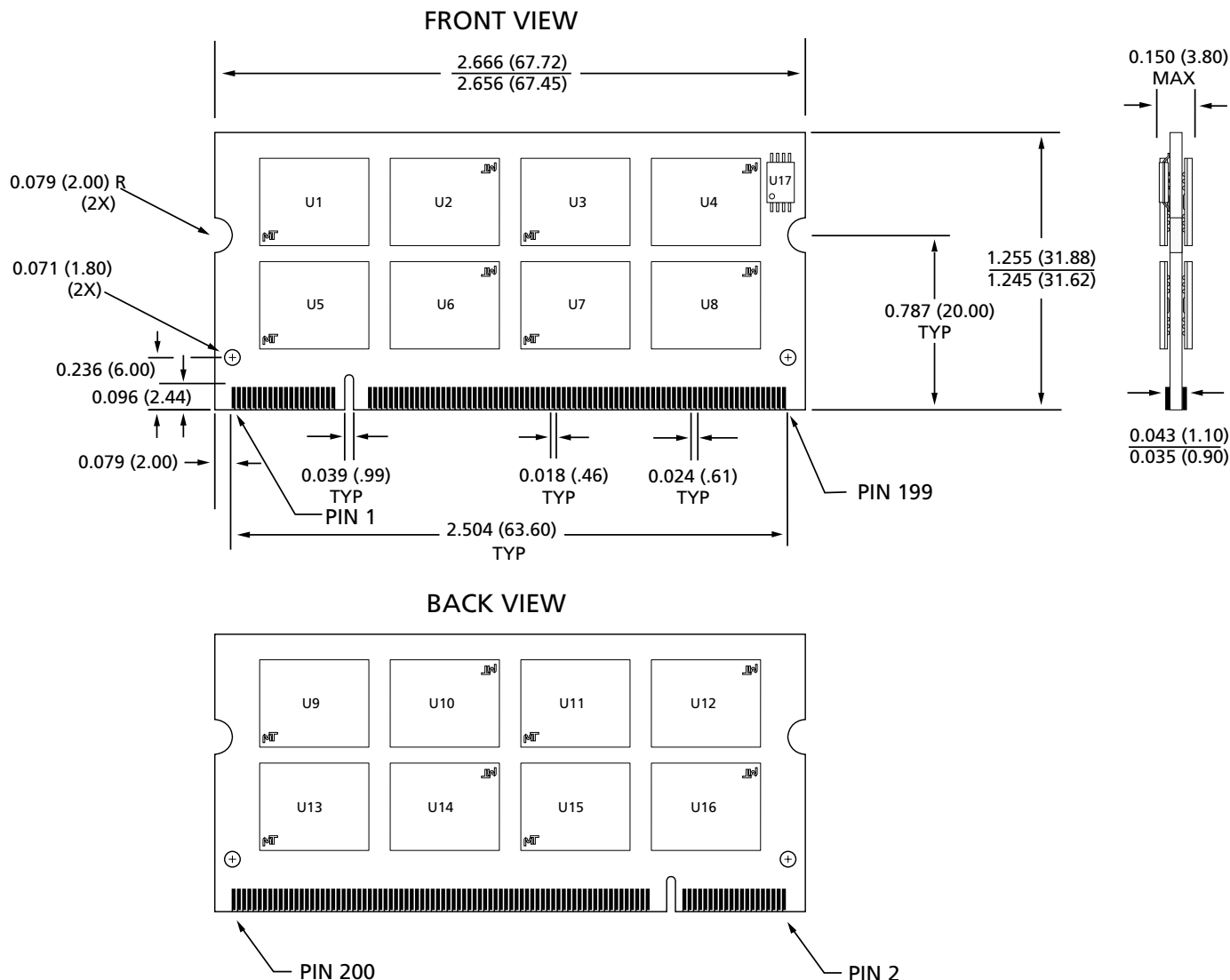
Figure 16: 200-PIN SODIMM Dimensions – 1GB
