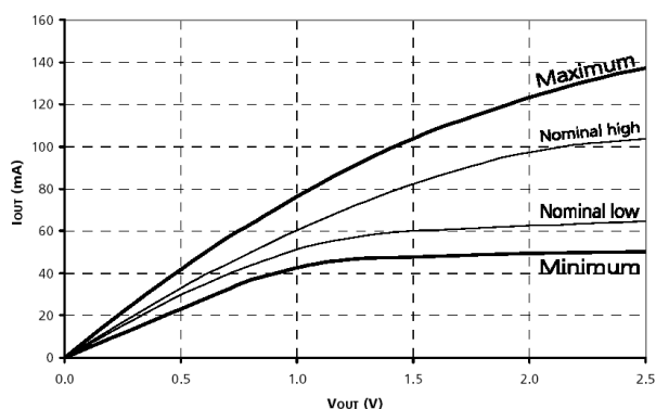
Figure 9: Pull-Down Characteristics
