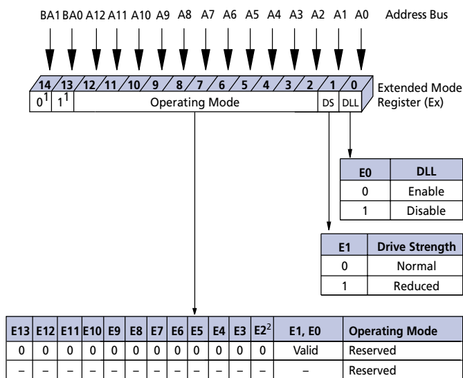
Figure 7: Extended Mode Register Definition Diagram
