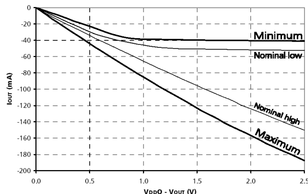
Figure 10: Pull-Up Characteristics
