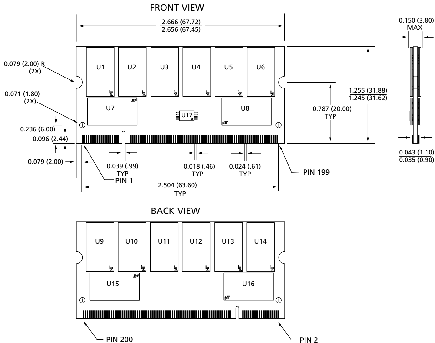
Figure 15: 200-PIN SODIMM Dimensions – 512MB
