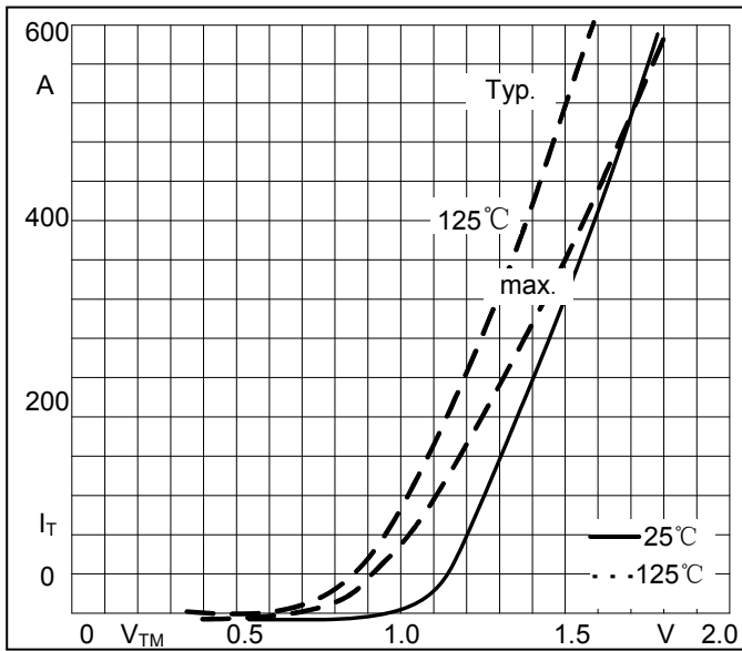
Fig5. Forward Characteristics
