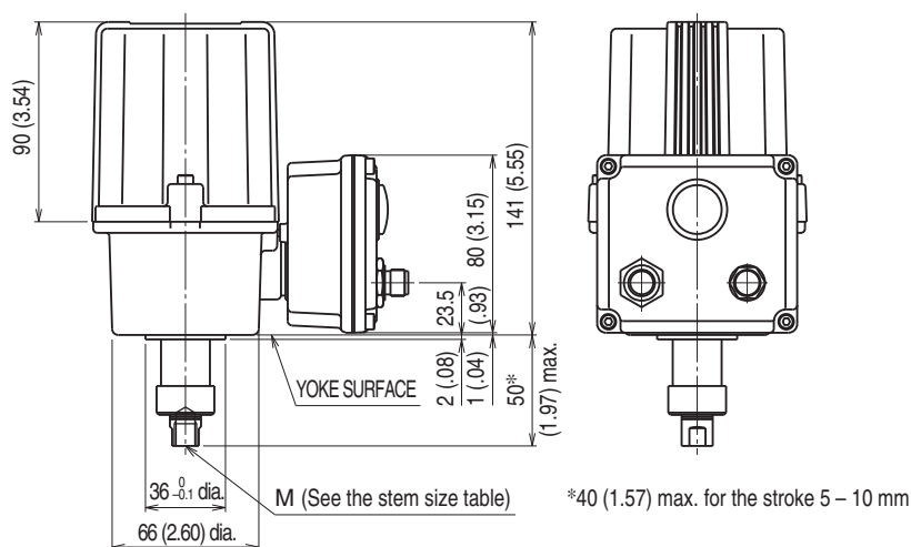
YOKE CONNECTION
