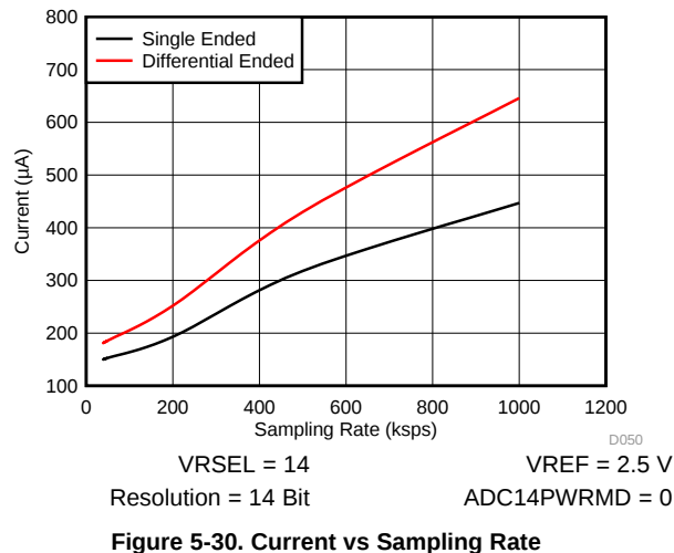
Figure 5-30. Current vs Sampling Rate
