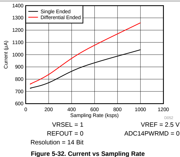
Figure 5-32. Current vs Sampling Rate
