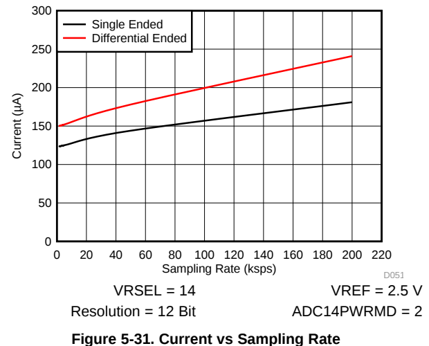
Figure 5-31. Current vs Sampling Rate
