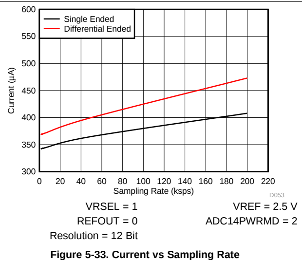
Figure 5-33. Current vs Sampling Rate
