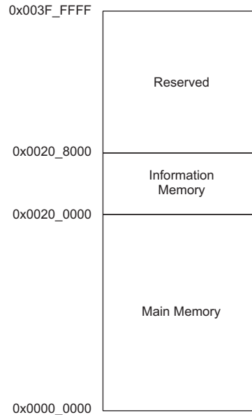
Figure 6-5. Flash Memory Map
