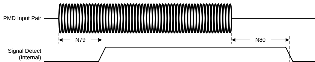
Figure 5-44. 100Base-TX Signal Detect Timing
