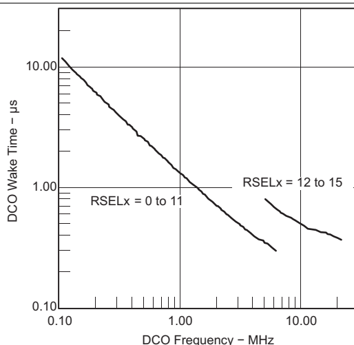
Figure 5-18. DCO Wake-up Time From LPM3 vs DCO Frequency
