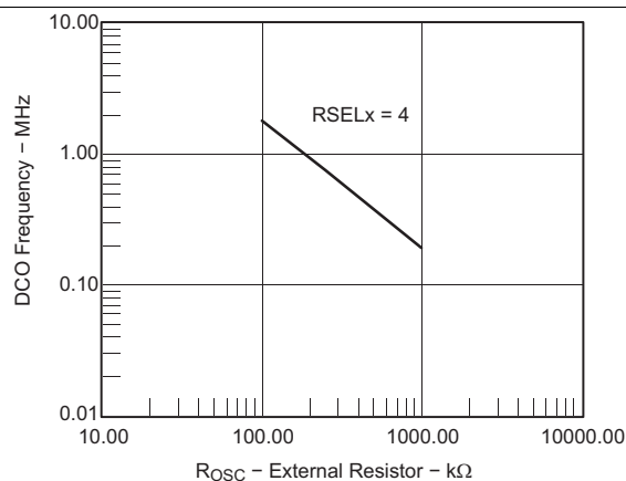
Figure 5-19. DCO Frequency vs R osc (V CC = 2.2 V, T A = 25°C)
