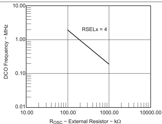
Figure 5-20. DCO Frequency vs R osc (V CC = 3 V, T A = 25°C)
