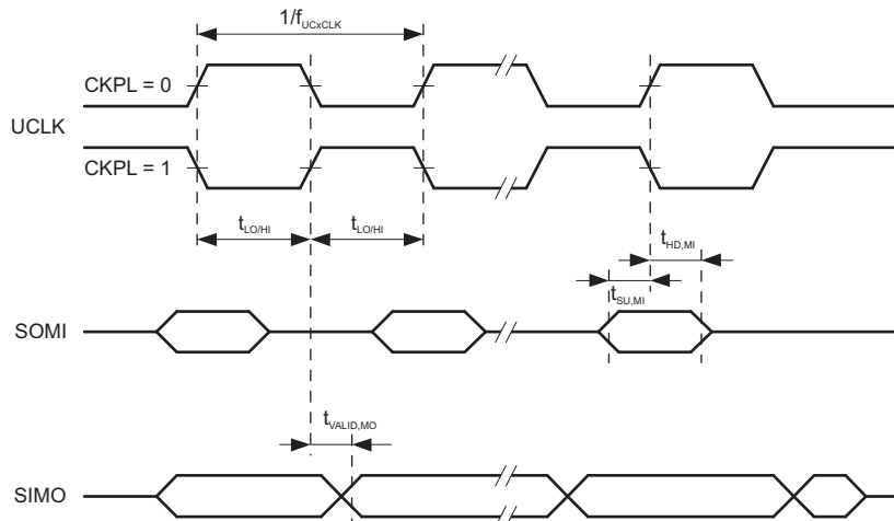
Figure 5-28. SPI Master Mode, CKPH = 1
