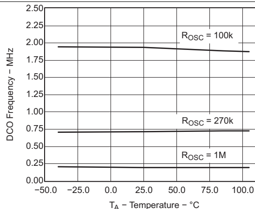
Figure 5-21. DCO Frequency vs Temperature (V CC = 3 V)
