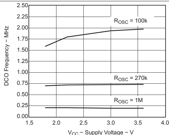
Figure 5-22. DCO Frequency vs Supply Voltage (T A = 25°C)
