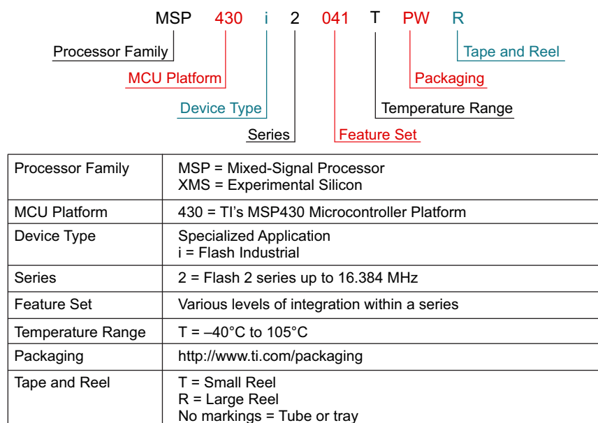
Figure 8-1. Device Nomenclature
