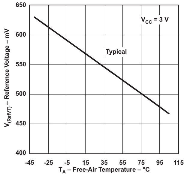
Figure 22. V_{(RefVT)} vs Temperature, V_{CC} = 3\text{ V}
