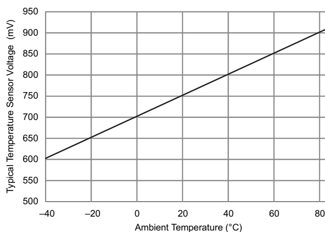
Figure 5-20. Typical Temperature Sensor Voltage
