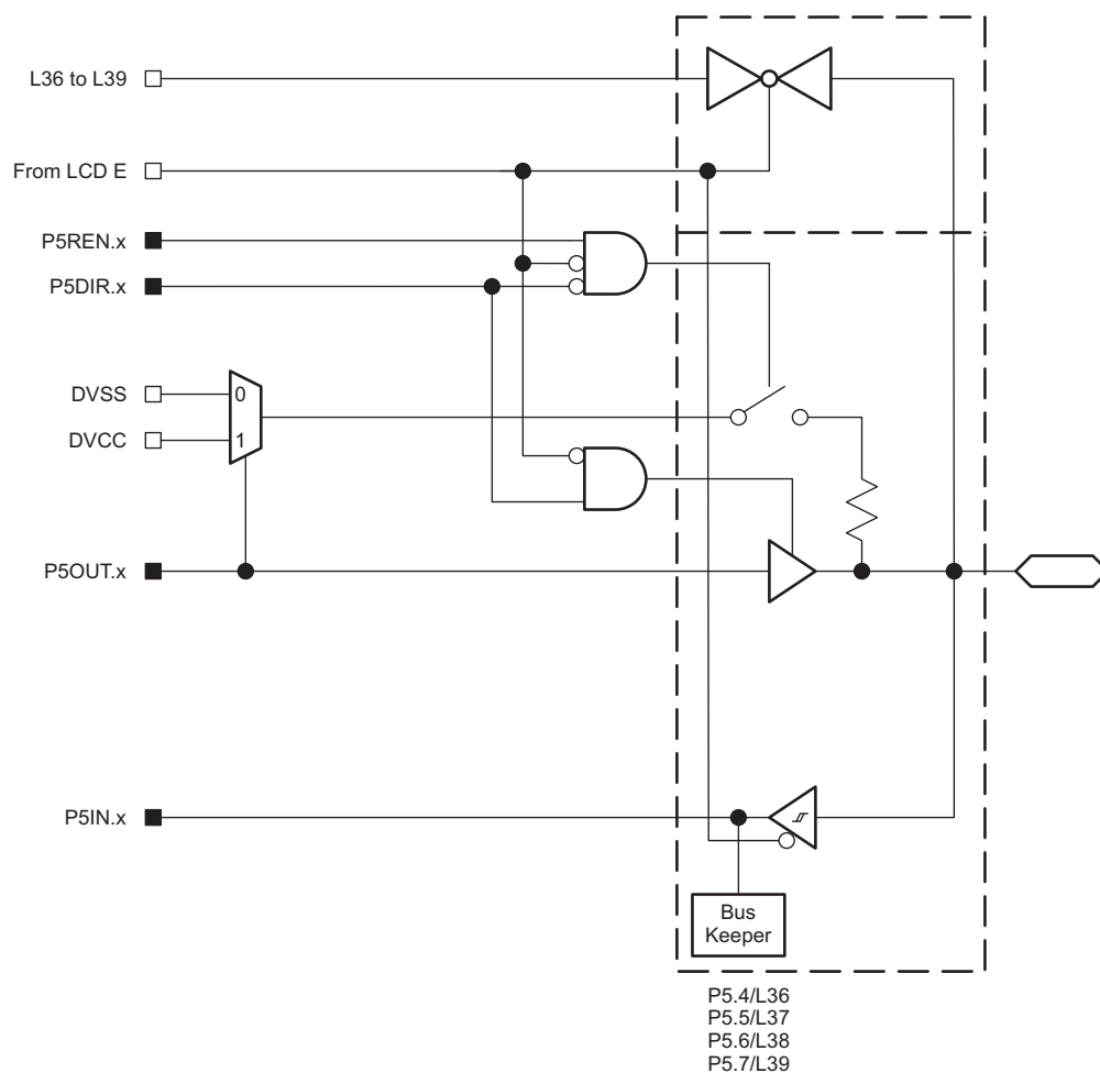
Figure 6-10. Port P5.4, P5.5, P5.6, and P5.7 Input/Output With Schmitt Trigger
