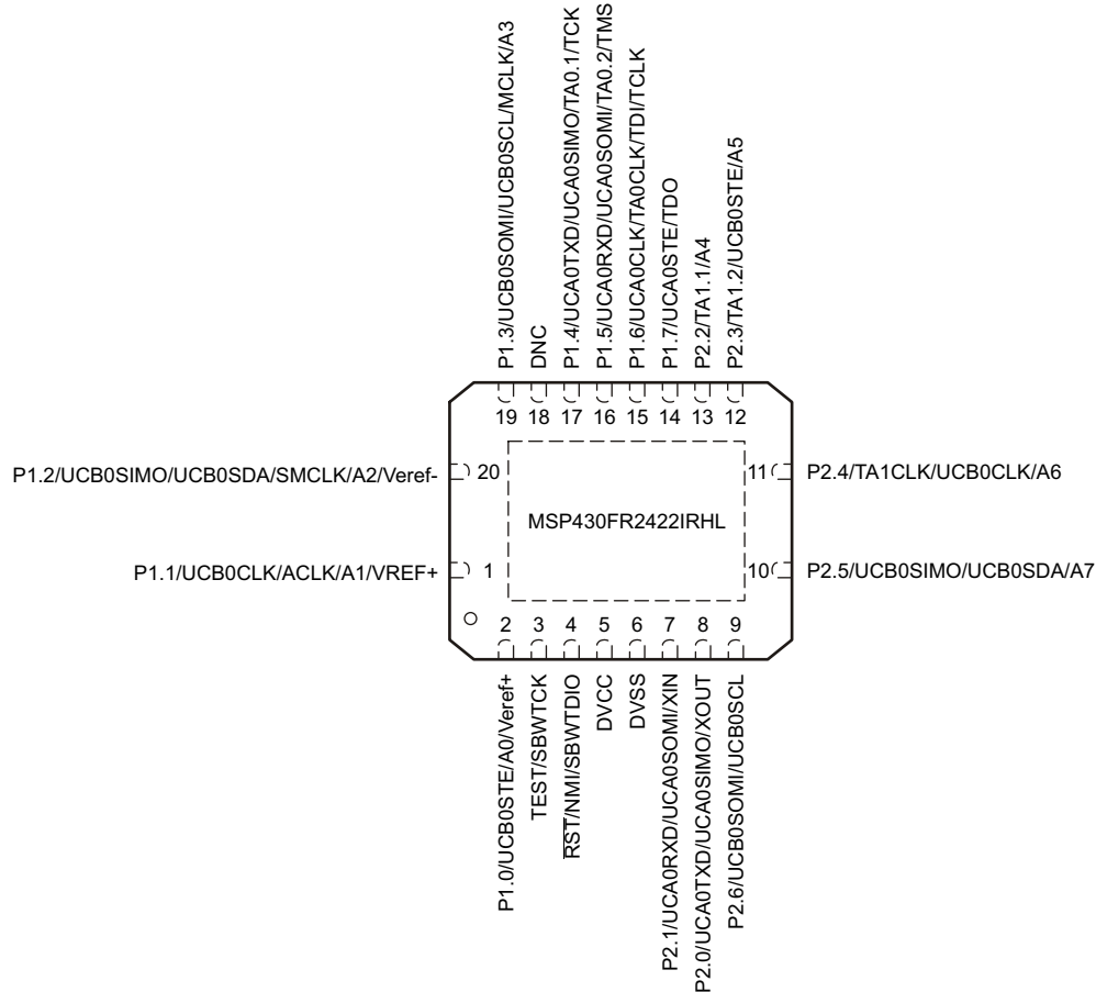
Figure 4-1. 20-Pin RHL Package (Top View)
