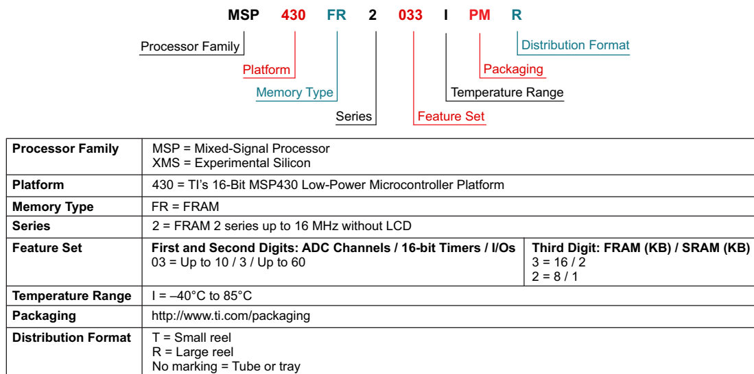
Figure 8-1. Device Nomenclature
