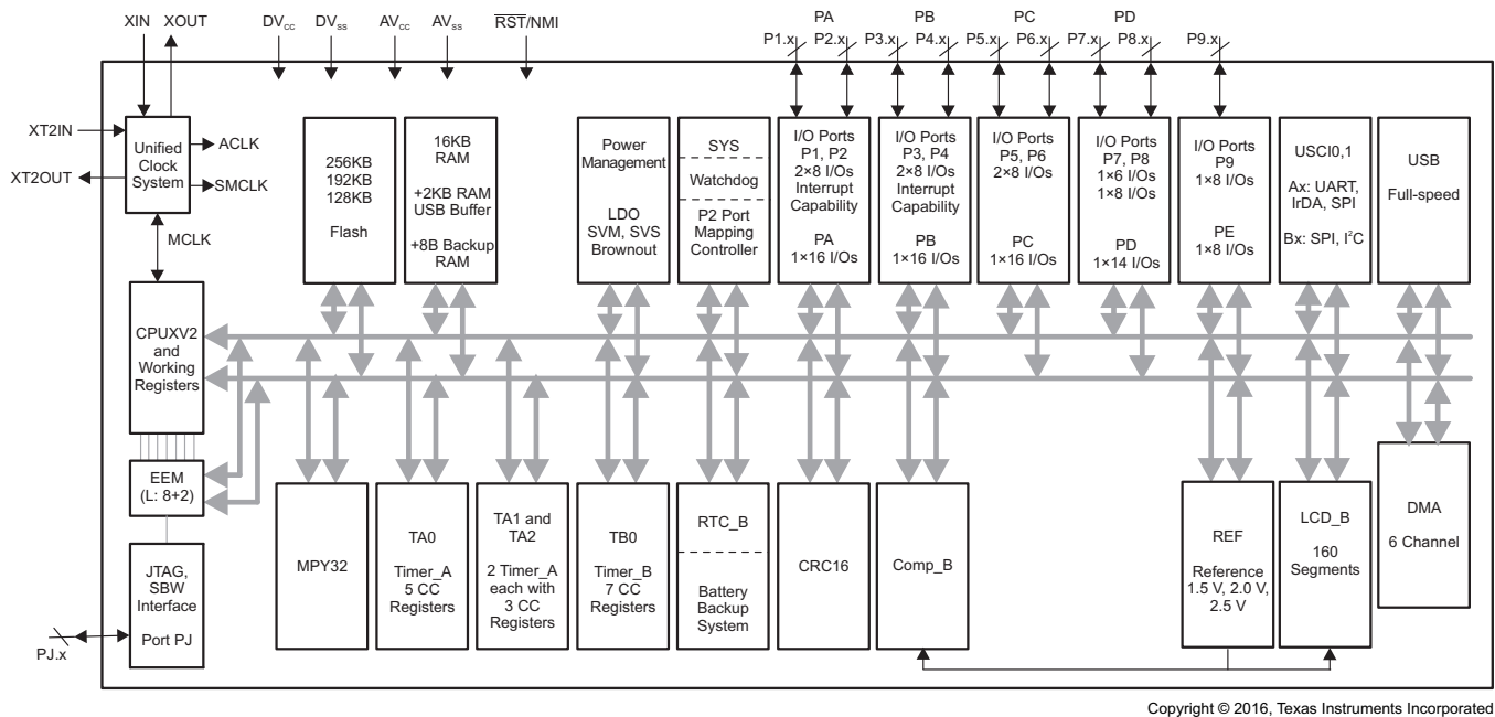
Figure 1-3. Functional Block Diagram – MSP430F6632, MSP430F6631, MSP430F6630
