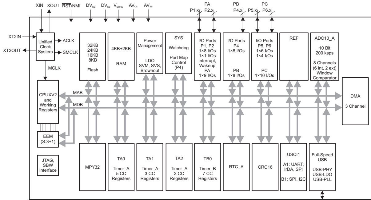
Figure 1-3. Functional Block Diagram – RGZ or PT Package – MSP430F5507, MSP430F5506, MSP430F5505, MSP430F5504
