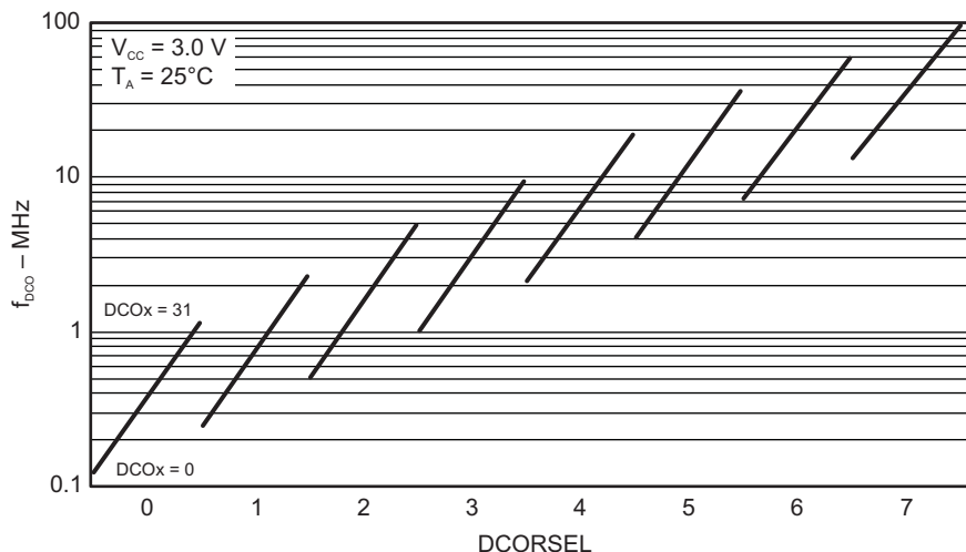
Figure 5-11. Typical DCO Frequency
