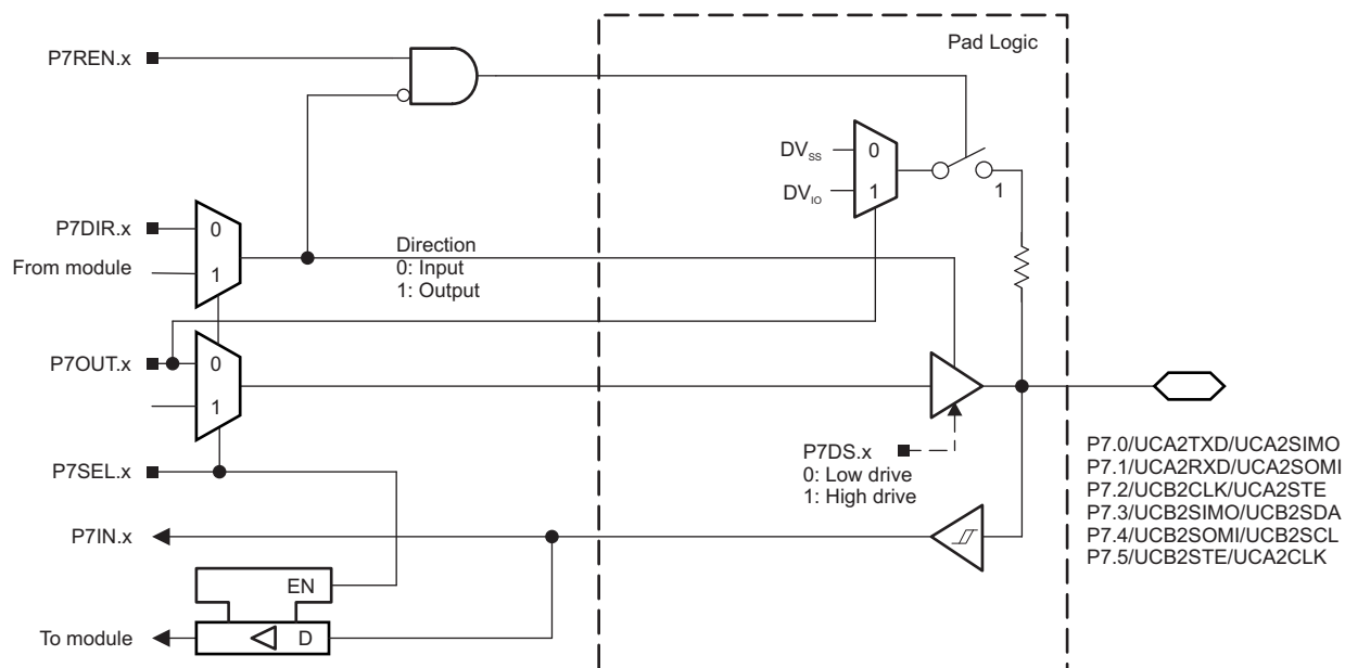
Figure 6-12. Port P7 (P7.0 to P7.5) Diagram
