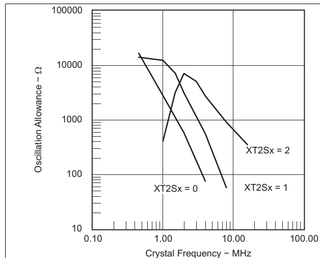
Figure 5-25. Oscillation Allowance vs Crystal Frequency C_{L,eff} = 15 \text{ pF} , T_A = 25^\circ\text{C}
