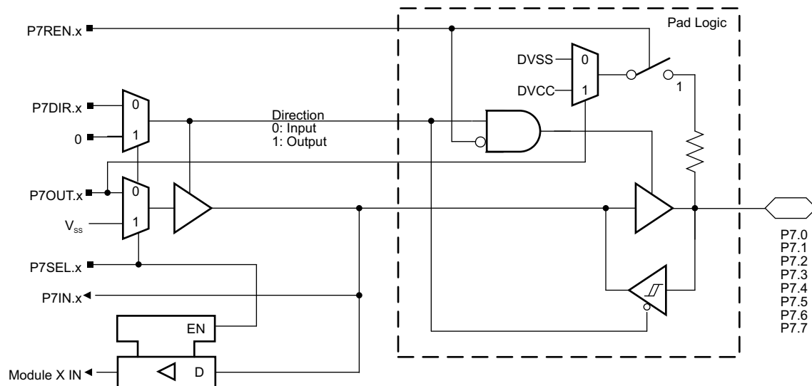
Figure 6-15. Port P7 (P7.0 to P7.7) Diagram
