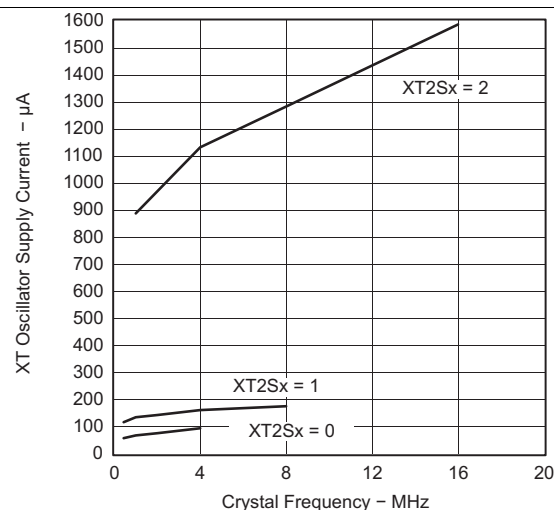
Figure 5-26. Oscillator Supply Current vs Crystal Frequency C_{L,eff} = 15 \text{ pF} , T_A = 25^\circ\text{C}
