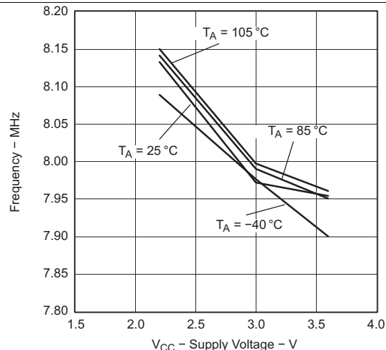
Figure 5-15. Calibrated 8-MHz Frequency vs Supply Voltage
