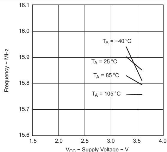
Figure 5-17. Calibrated 16-MHz Frequency vs Supply Voltage
