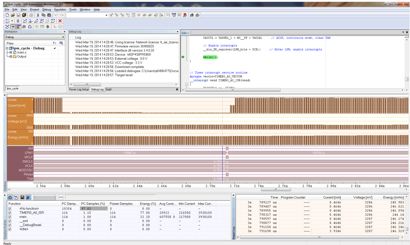
Figure 11. Debug Session With EnergyTrace++ Windows
