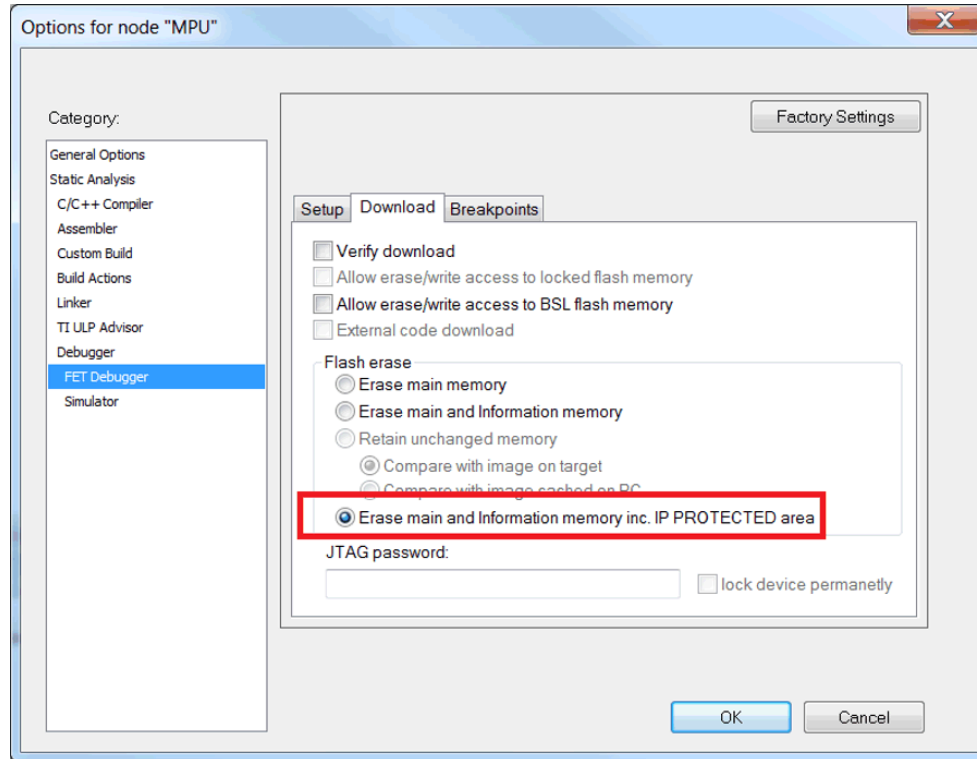
Figure 33. IPE Debug Settings
