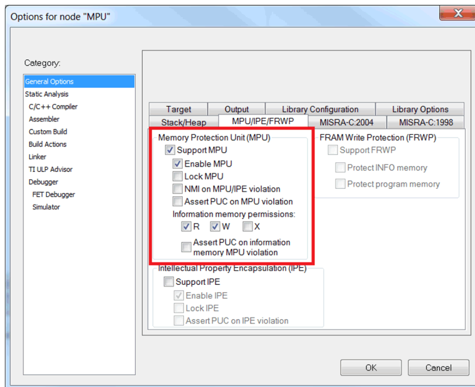
Figure 31. MPU Configuration Dialog
