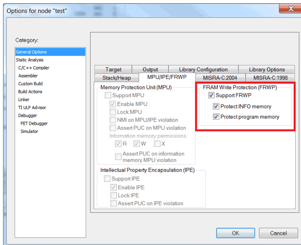
Figure 34. FRWP Configuration Dialog
