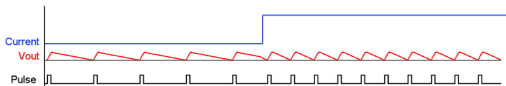
Figure 10. Pulse Density and Current Flow
