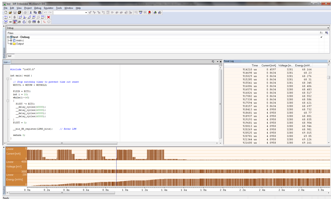
Figure 22. Debug Session With EnergyTrace Windows
