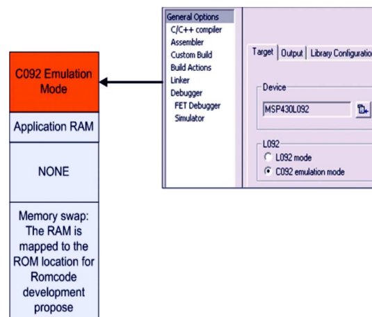
Figure 4. C092 Emulation Mode
