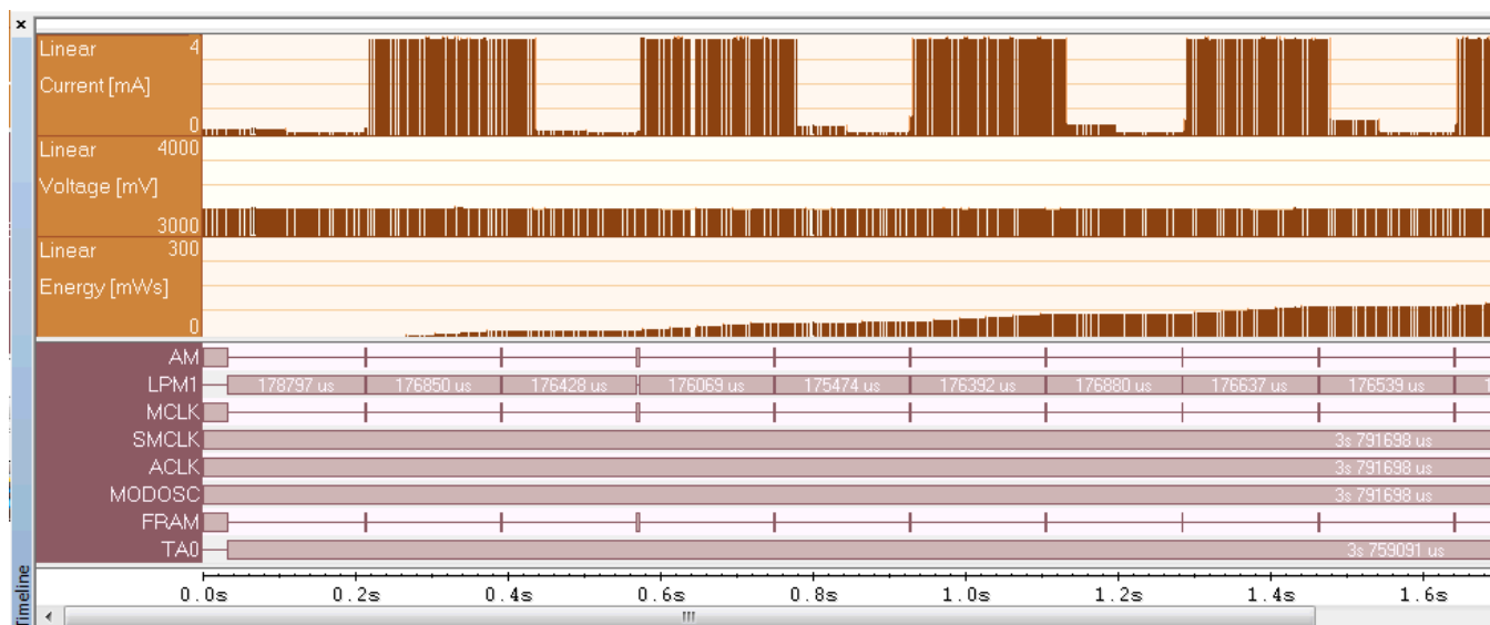
Figure 20. Timeline With EnergyTrace++ Data
