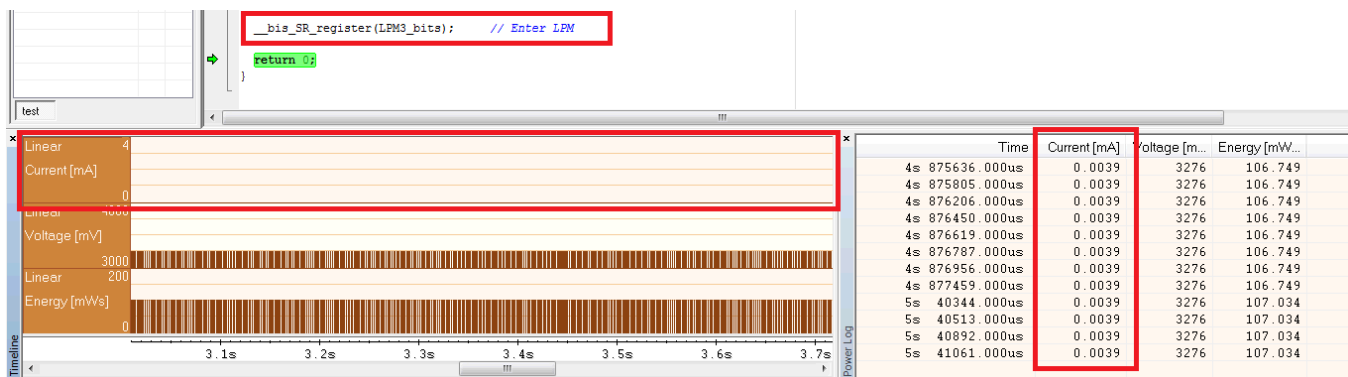
Figure 30. LPM3 Current When Executing with JTAG Signals Released
