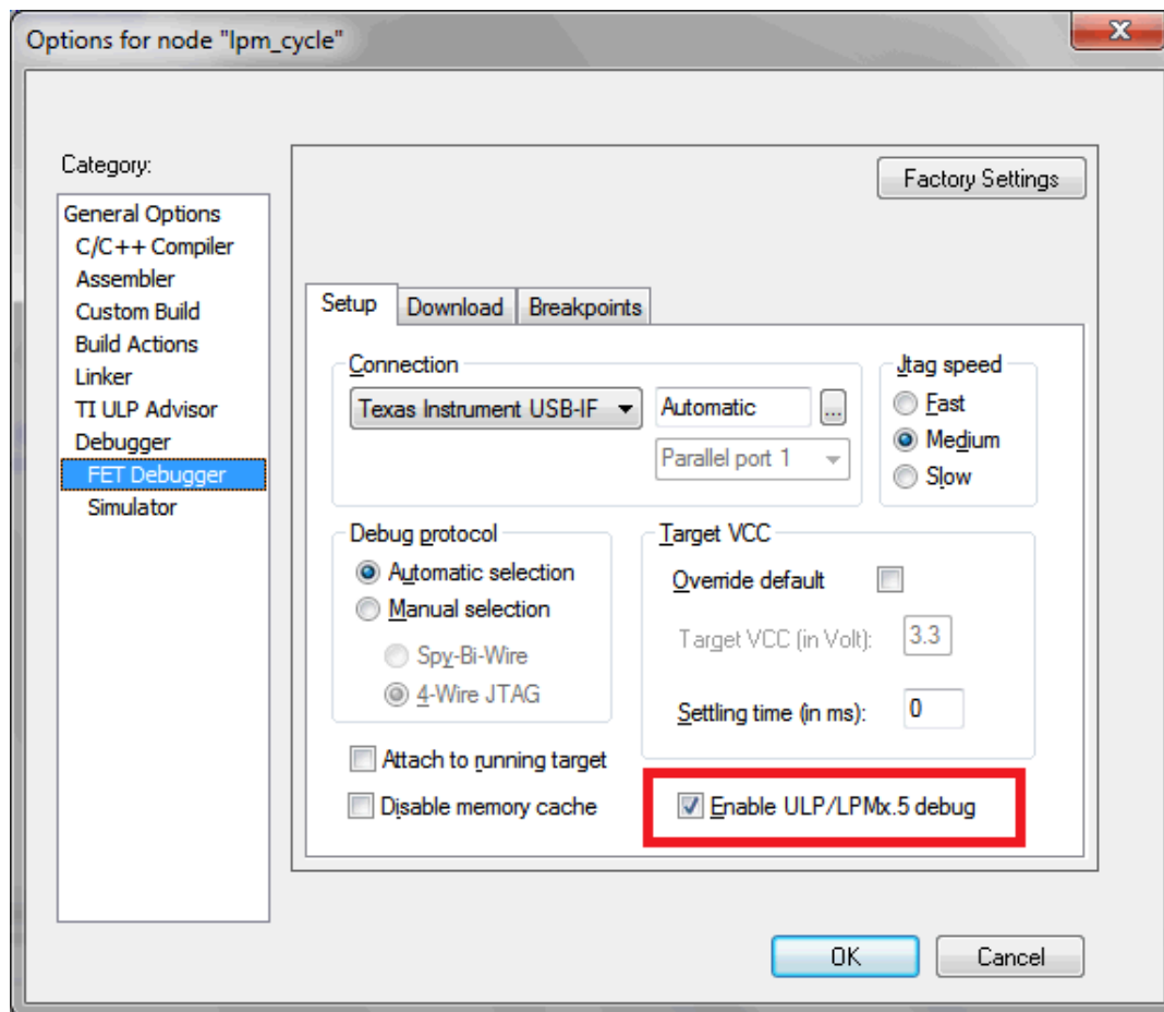
Figure 12. Debug Options
