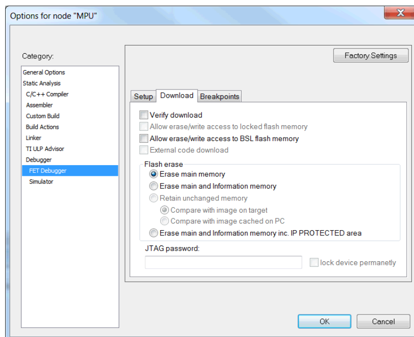
Figure 8. Download Options
