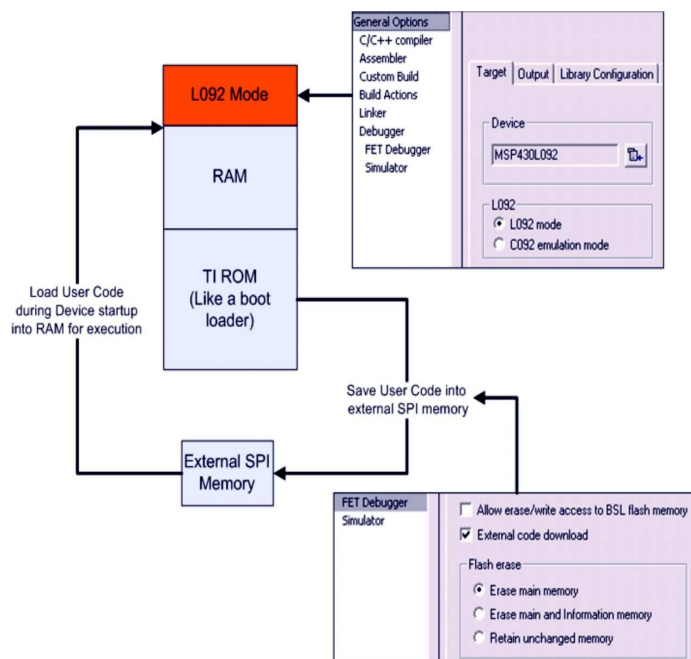
Figure 3. L092 Mode
