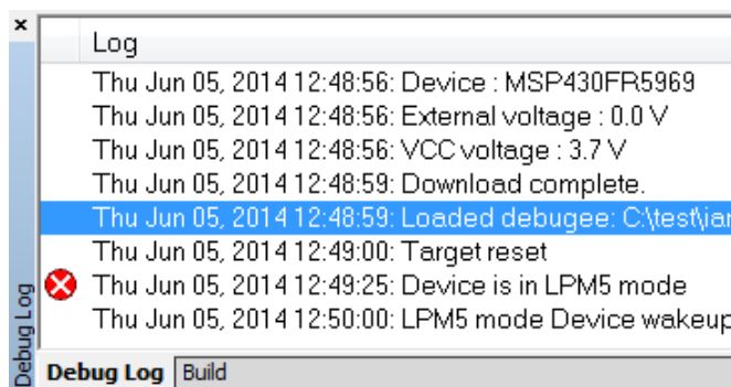
Figure 7. LPMx.5 Notifications
