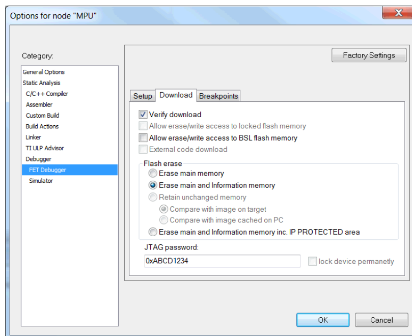
Figure 9. JTAG Password
