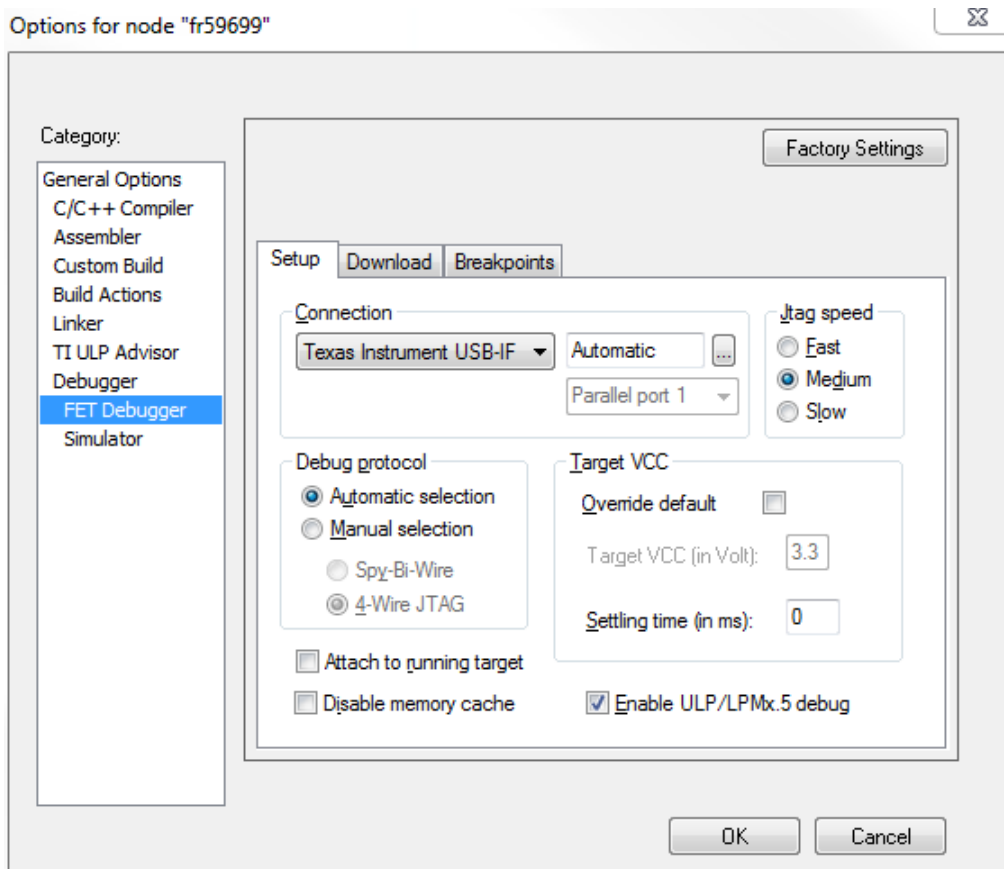
Figure 6. Enable Ultra-Low-Power Debug Mode
