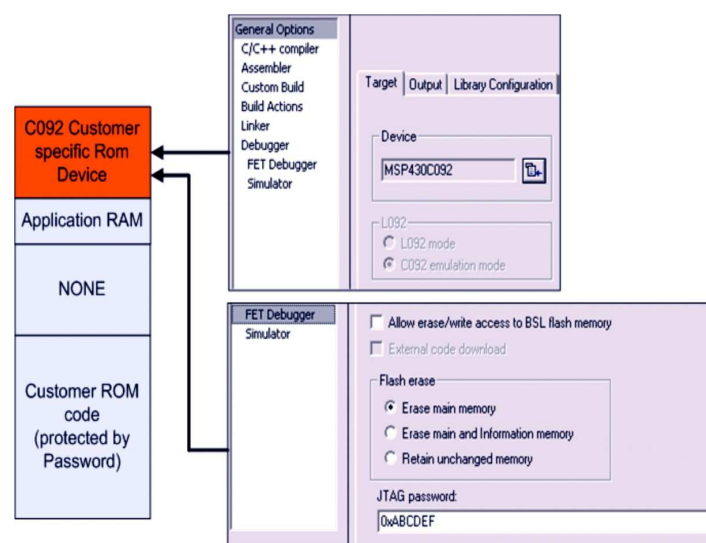
Figure 5. C092 Password
