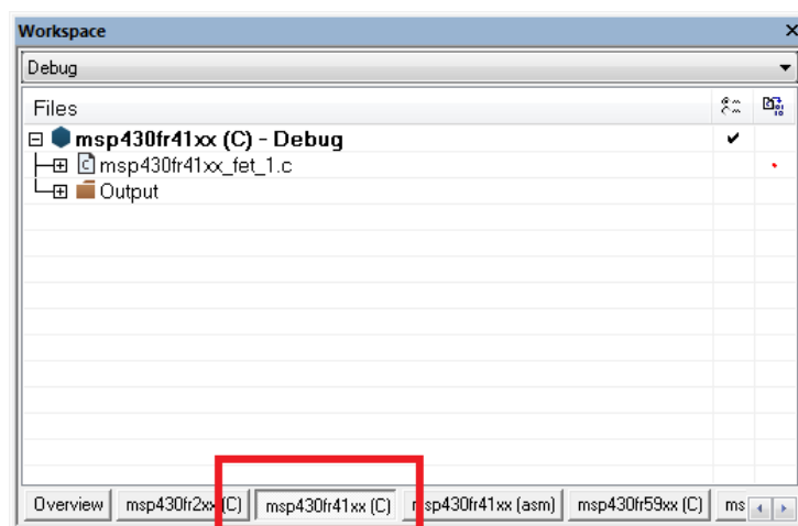
Figure 1. Activate Project
