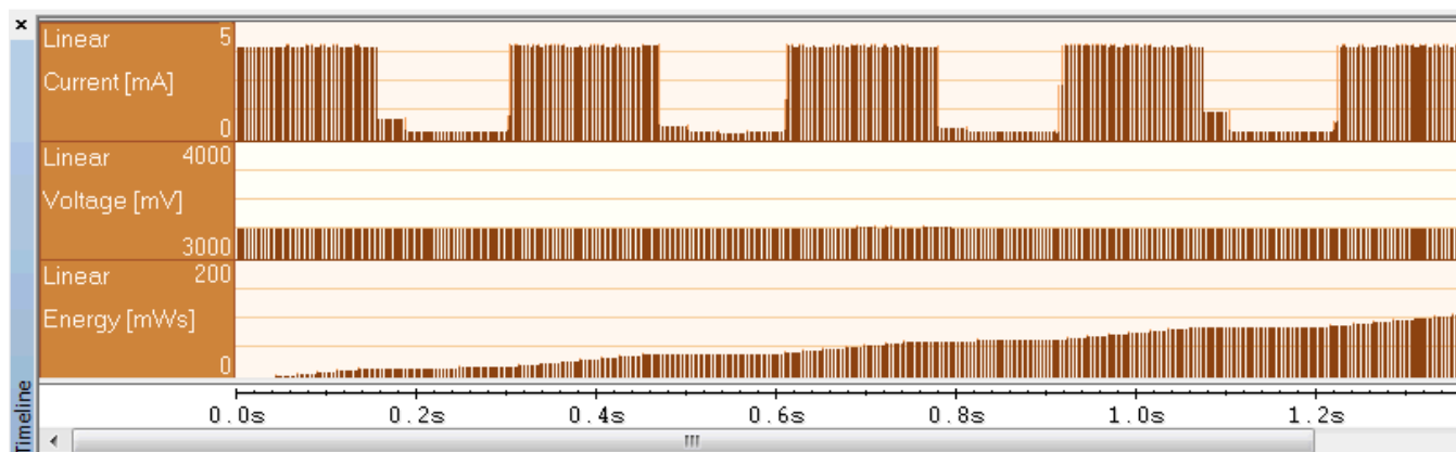
Figure 27. Timeline With EnergyTrace Data
