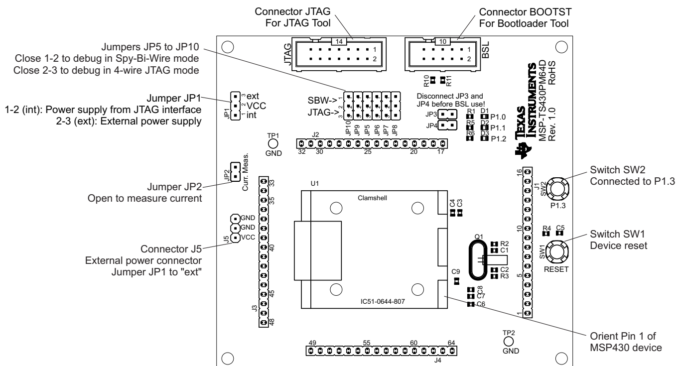
Figure B-49. MSP-TS430PM64D Target Socket Module, PCB
