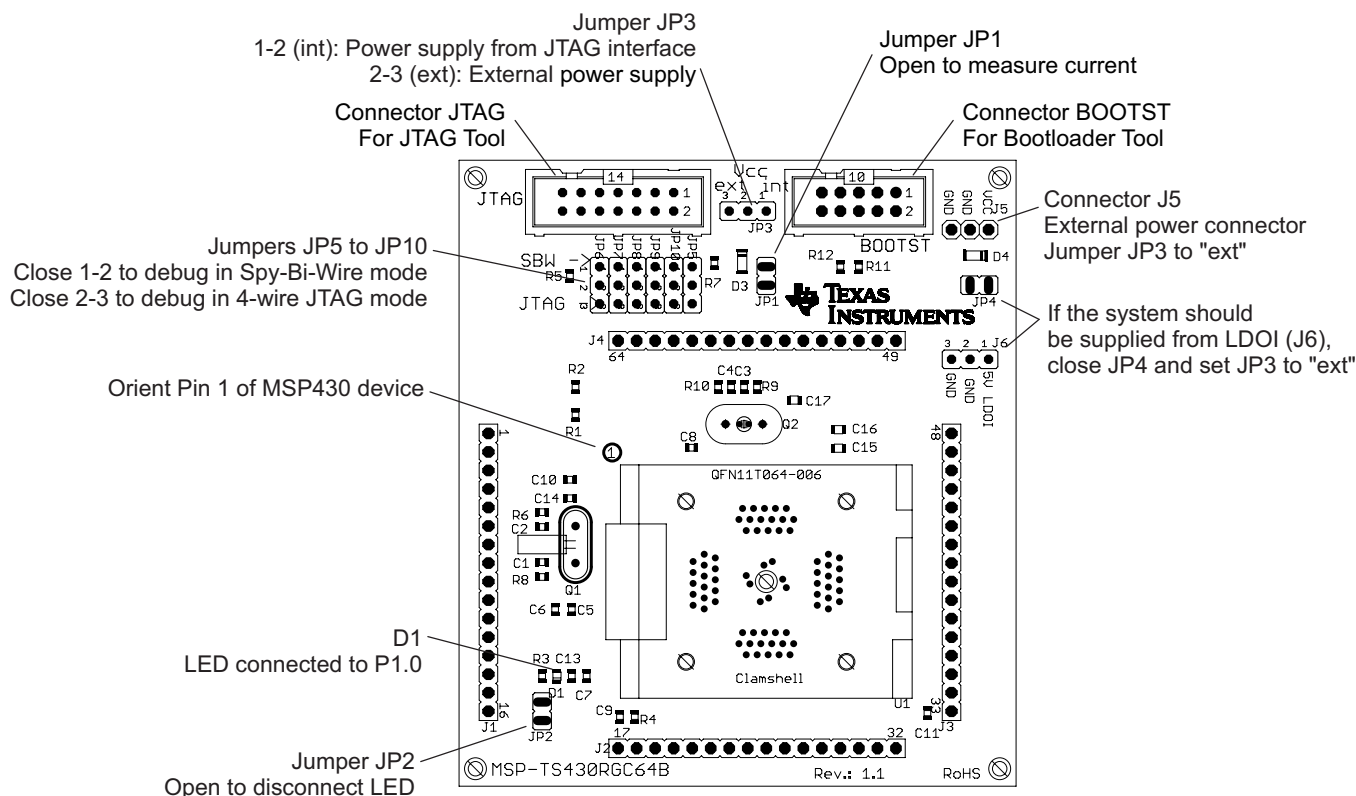
Figure B-53. MSP-TS430RGC64B Target Socket Module, PCB
