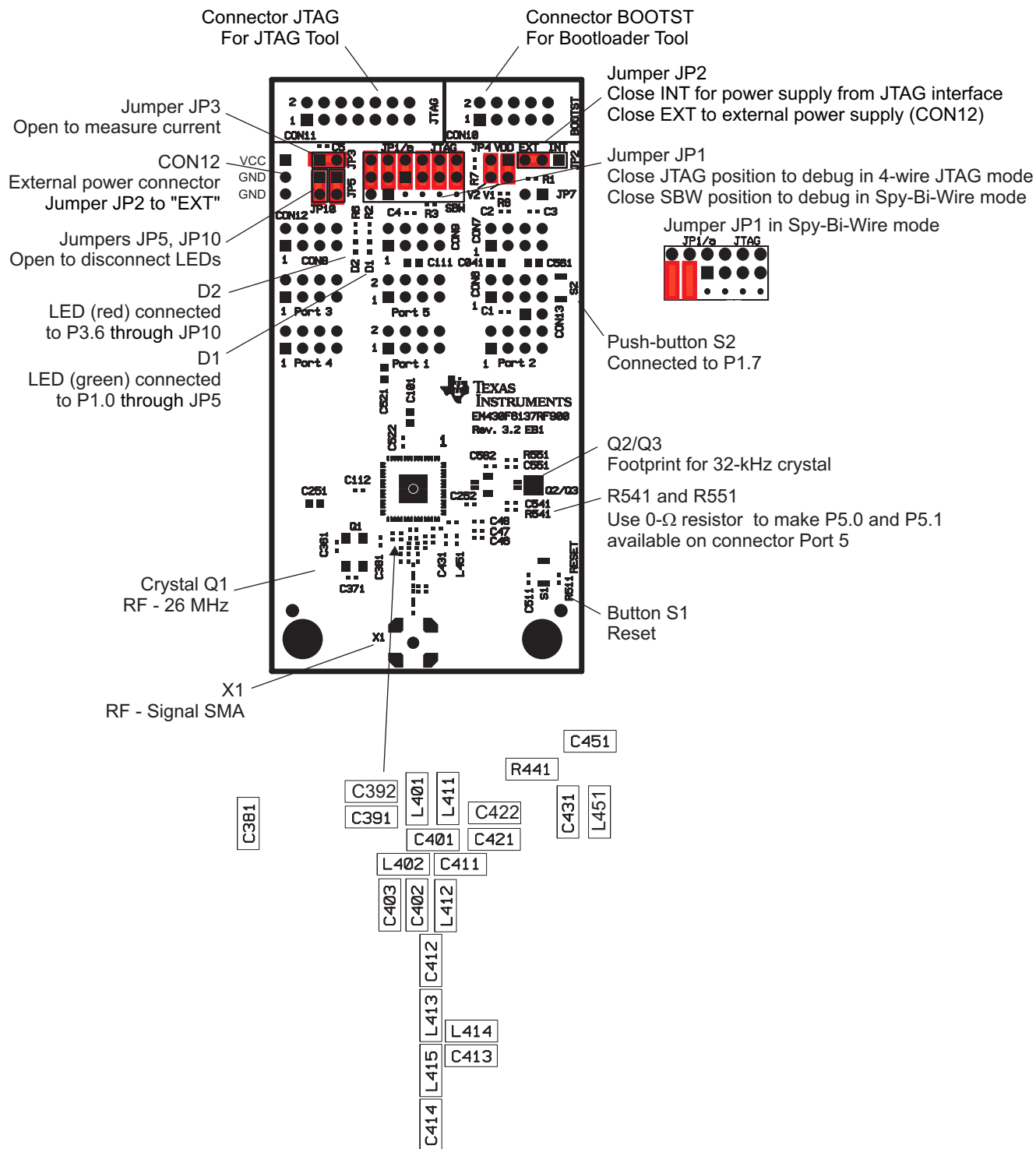
Figure B-91. EM430F6137RF900 Target Board, PCB
