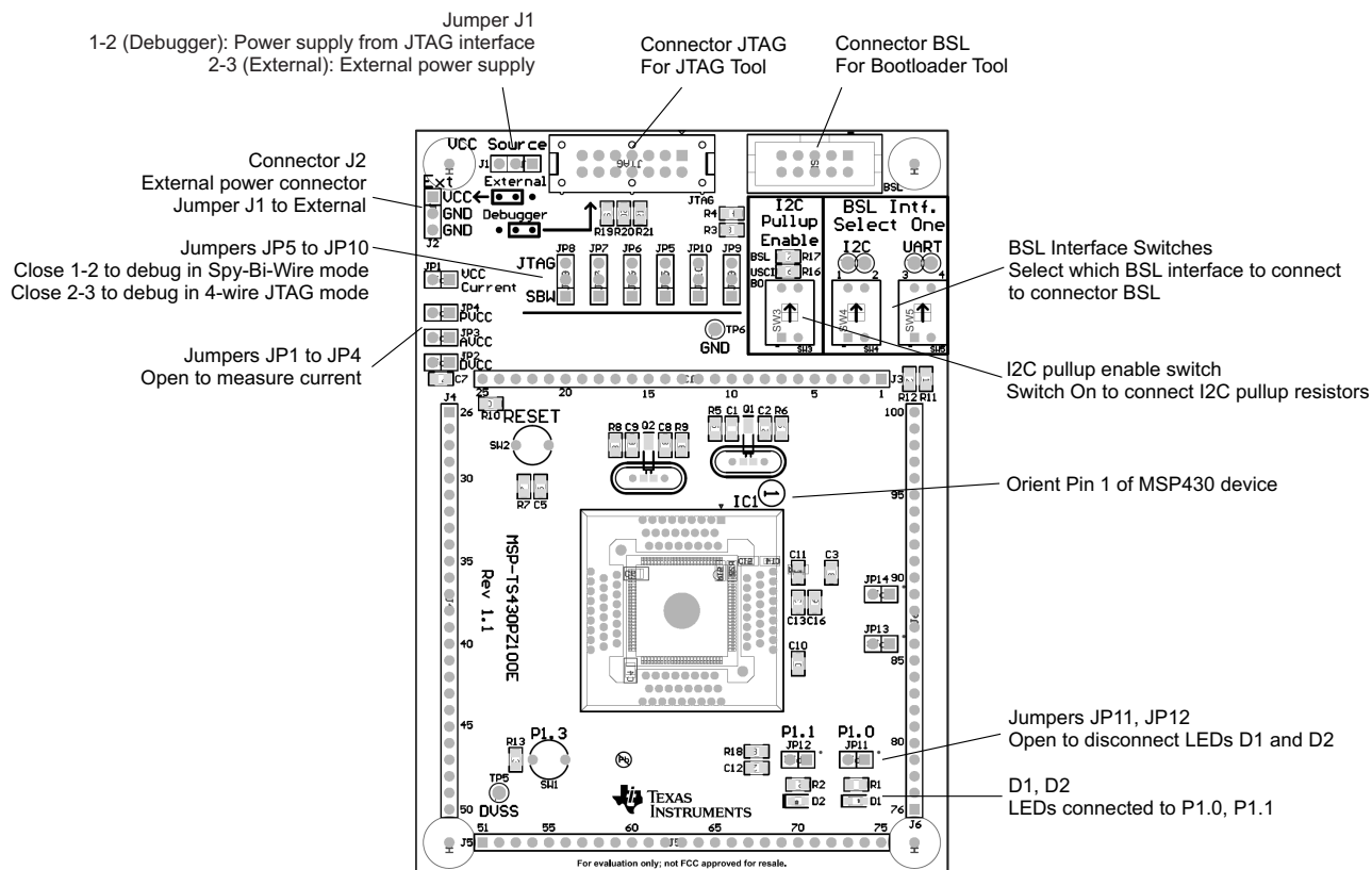
Figure B-79. MSP-TS430PZ100E Target Socket Module, PCB
