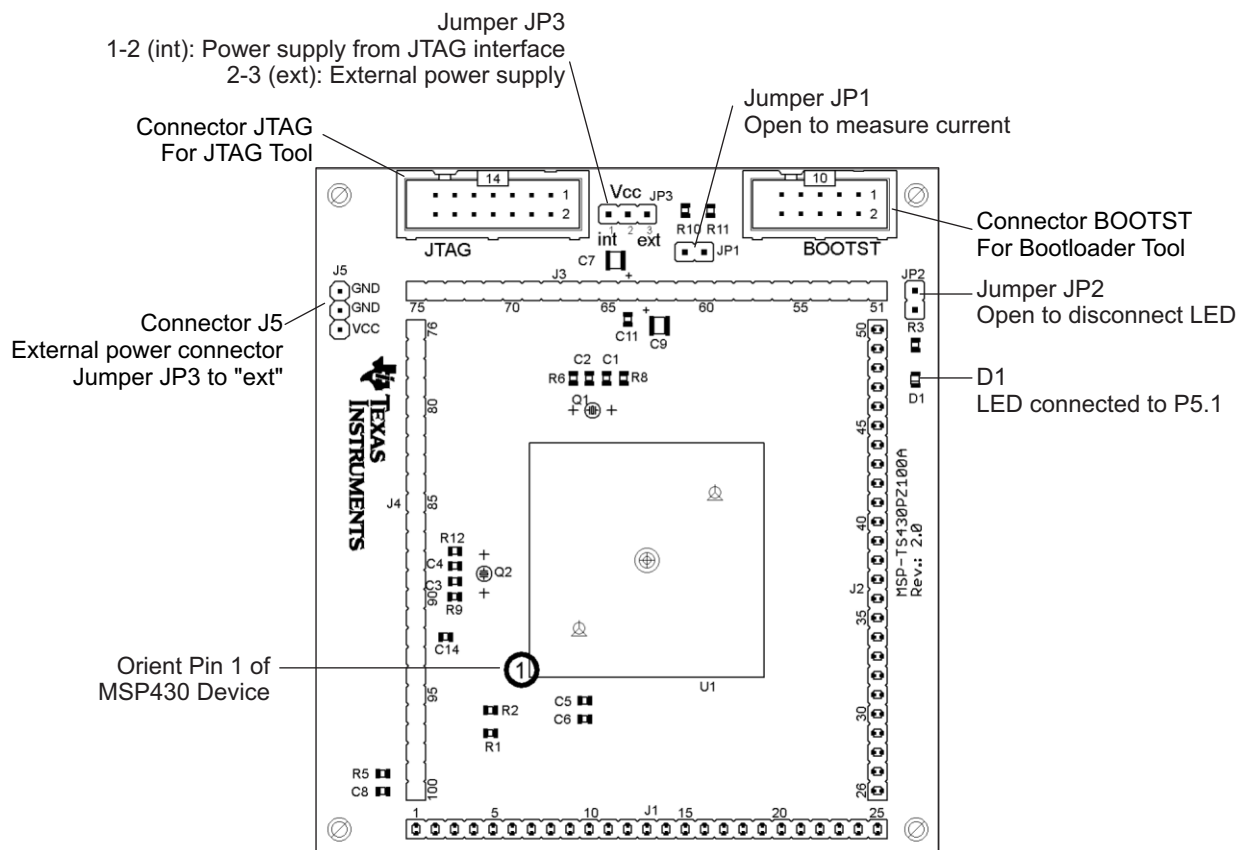
Figure B-71. MSP-TS430PZ100A Target Socket Module, PCB
