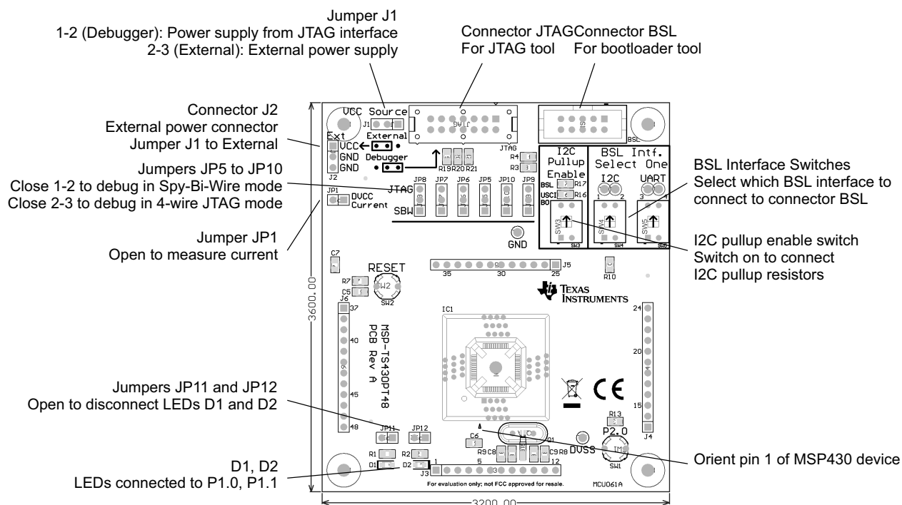
Figure B-37. MSP-TS430PT48 Target Socket Module, PCB
