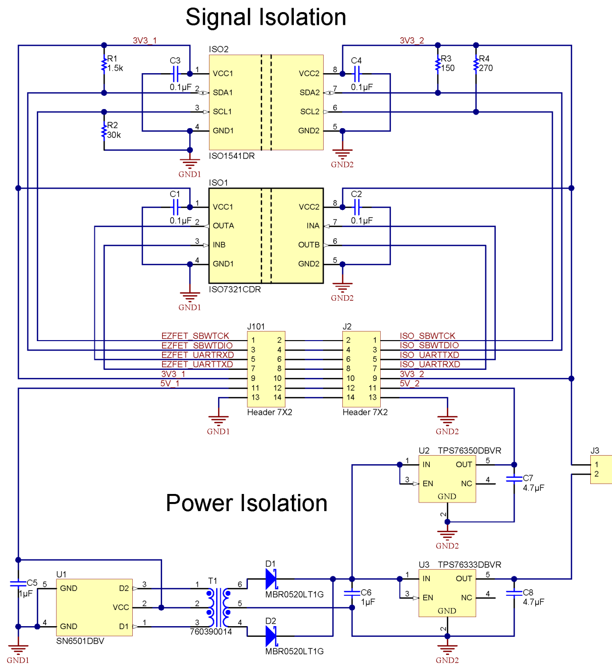
Figure 17. Schematics
