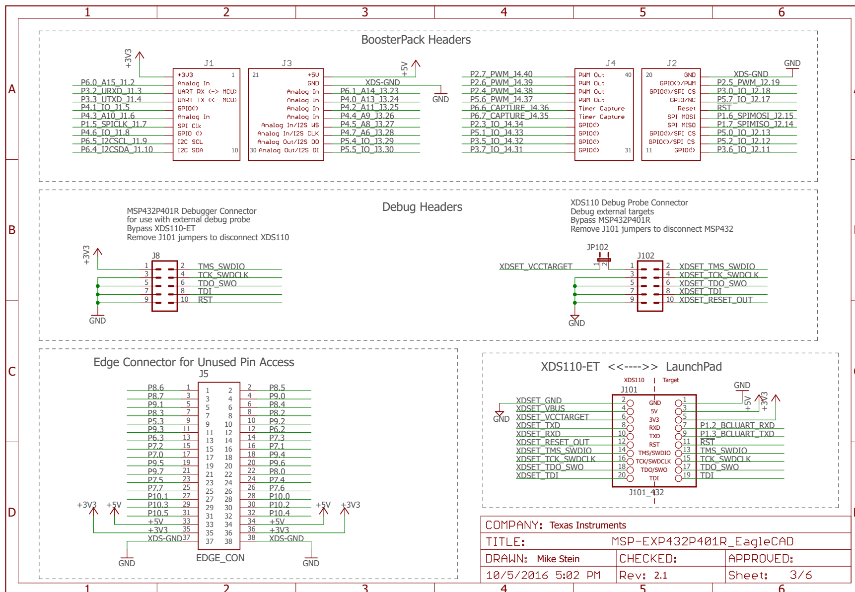
Figure 30. Schematics (3 of 6)
