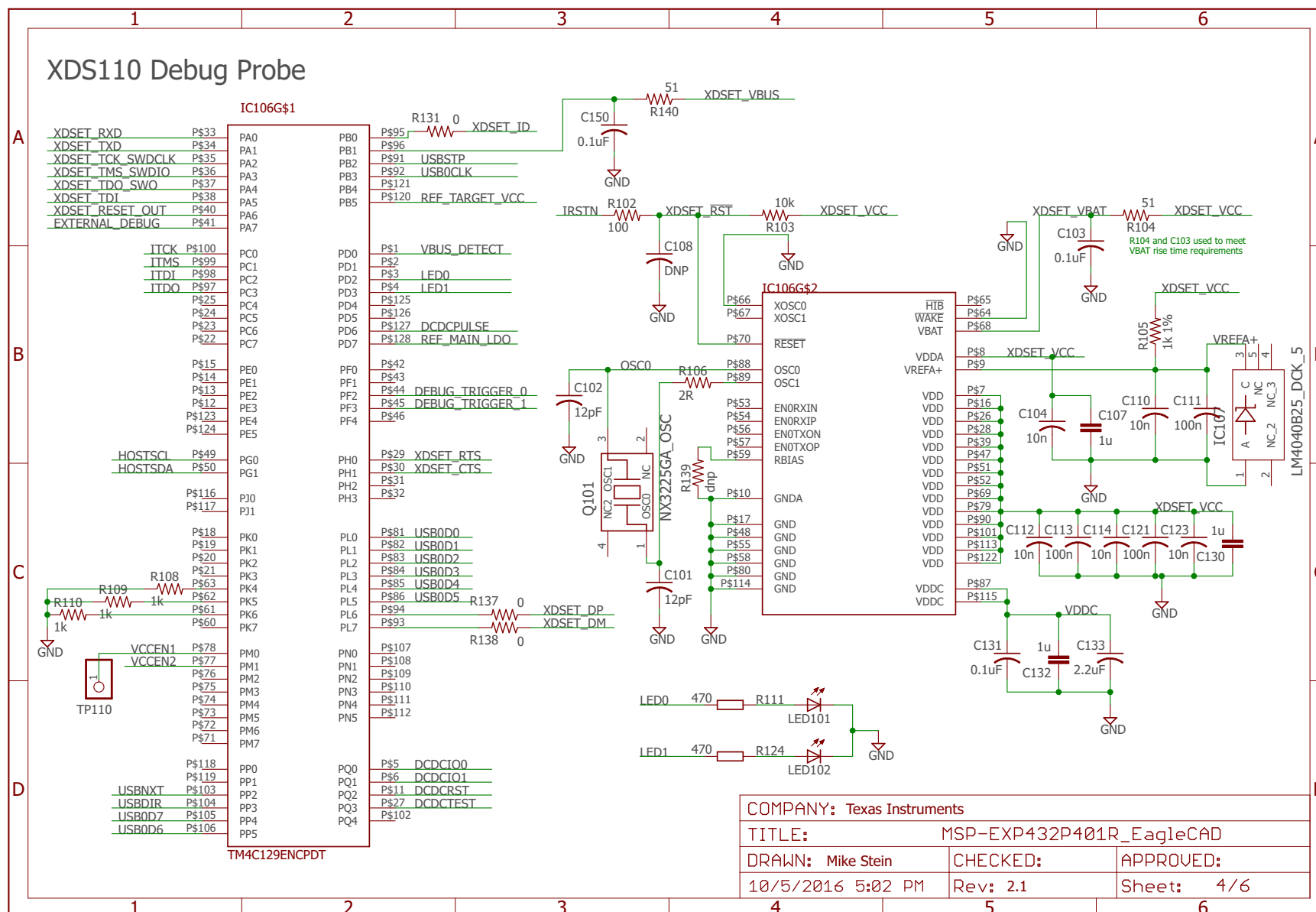
Figure 31. Schematics (4 of 6)
