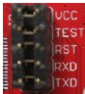
Figure 55. eZ430 Debug Connector on MSP-EXP430G2 LaunchPad
