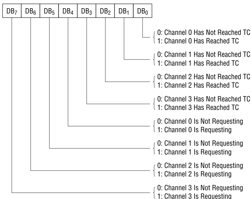
Figure 7 Status Register
