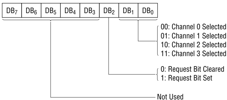
Figure 5 Request Register
