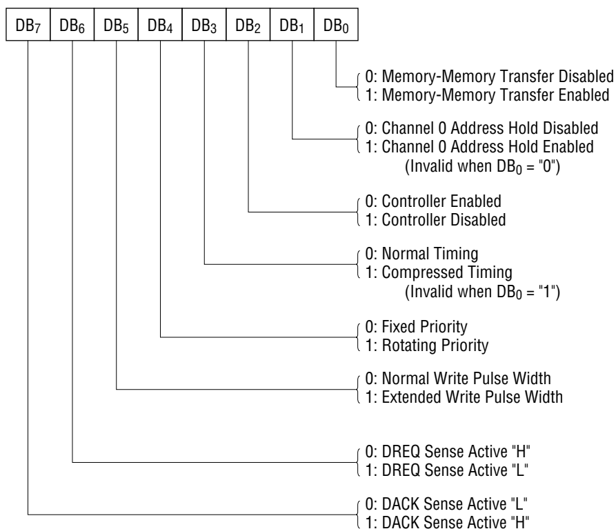
Figure 3 Command Register
