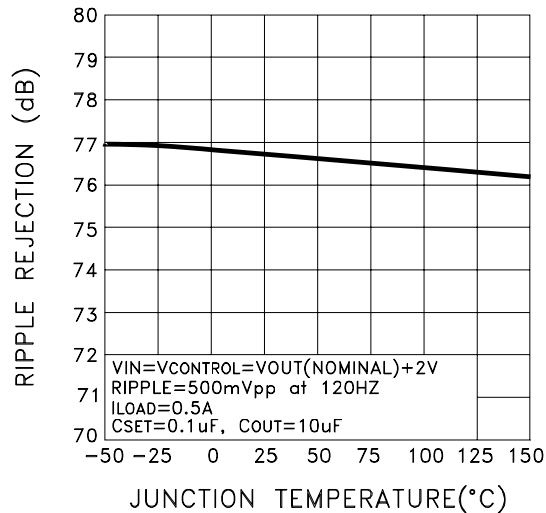
RIPPLE REJECTION (120Hz)
