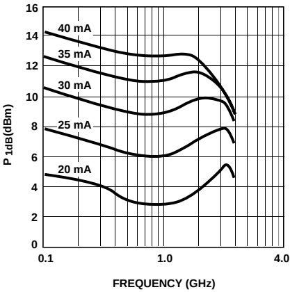
Figure 3. Typical P_{1dB} vs. Frequency at 25°C.
