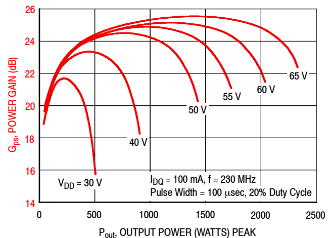
Figure 22. Power Gain versus Output Power and Drain-Source Voltage
