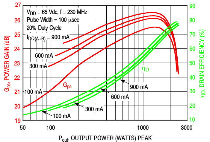
Figure 20. Power Gain and Drain Efficiency versus Output Power and Quiescent Current
