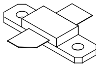
CASE 360B-05, STYLE 1 NI-360 MRF9045LR1
