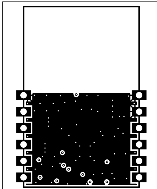
FIGURE 2-5: GROUND PLANE
