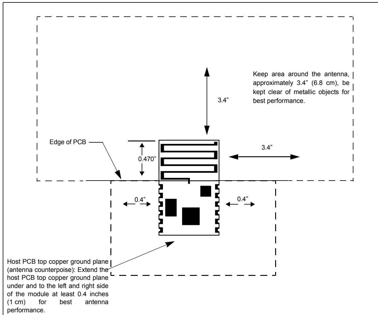
FIGURE 1-5: MOUNTING DETAILS
