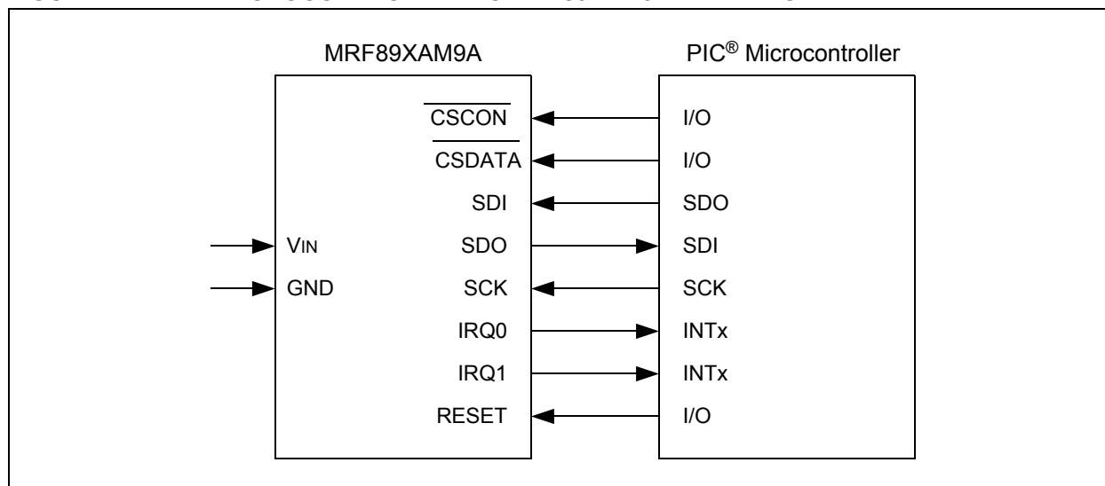
FIGURE 1-2: MICROCONTROLLER TO MRF89XAM9A INTERFACE
