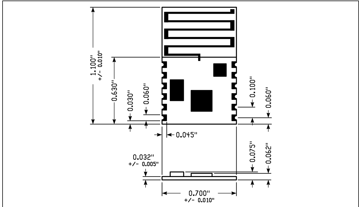
FIGURE 1-3: MODULE DETAILS
