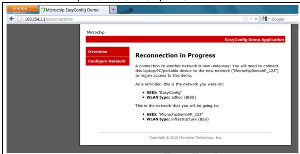
FIGURE 4-71: WEB BROWSER (COMPUTER 2): TRANSITION FROM OLD (AD HOC MODE) TO NEW (INFRASTRUCTURE MODE) NETWORK
