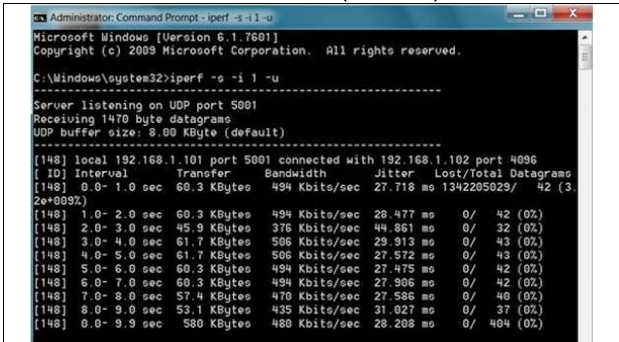
FIGURE 4-59: IPERF TRANSMIT PERFORMANCE (PC – SERVER)
