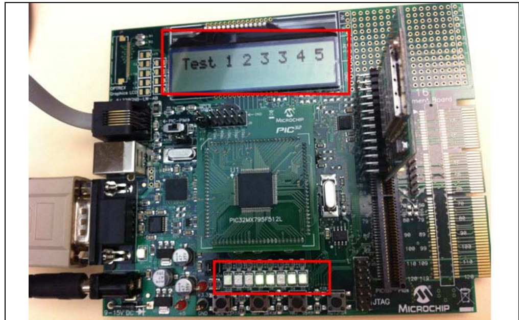
FIGURE 4-29: TCPIP – DEMO APPLICATION: LEDS AND LCD ON DEVELOPMENT BOARD
