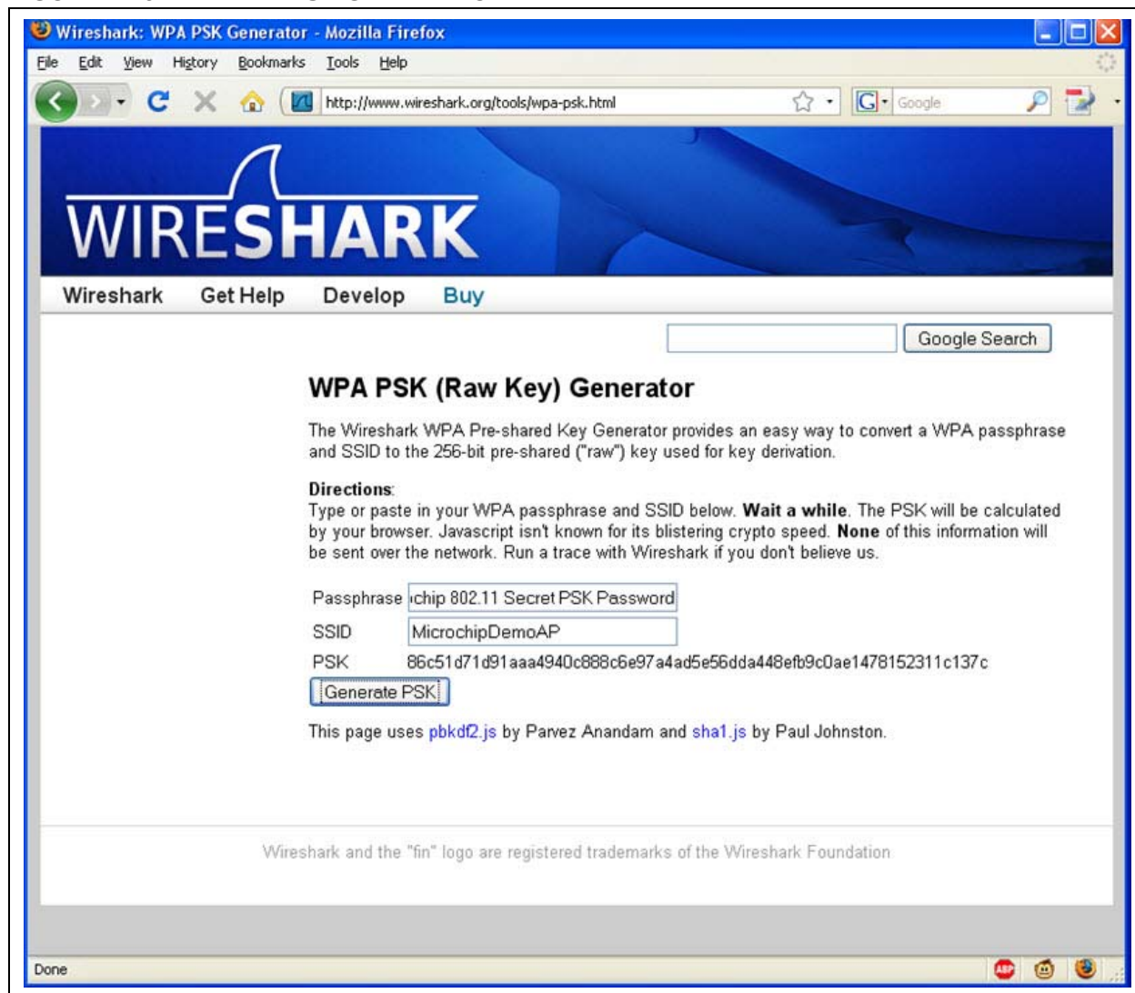
FIGURE 4-16: WPA PSK GENERATION
