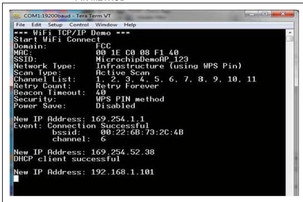
FIGURE 4-52: DEVELOPMENT BOARD SERIAL OUTPUT DISPLAY: WPS PIN METHOD
