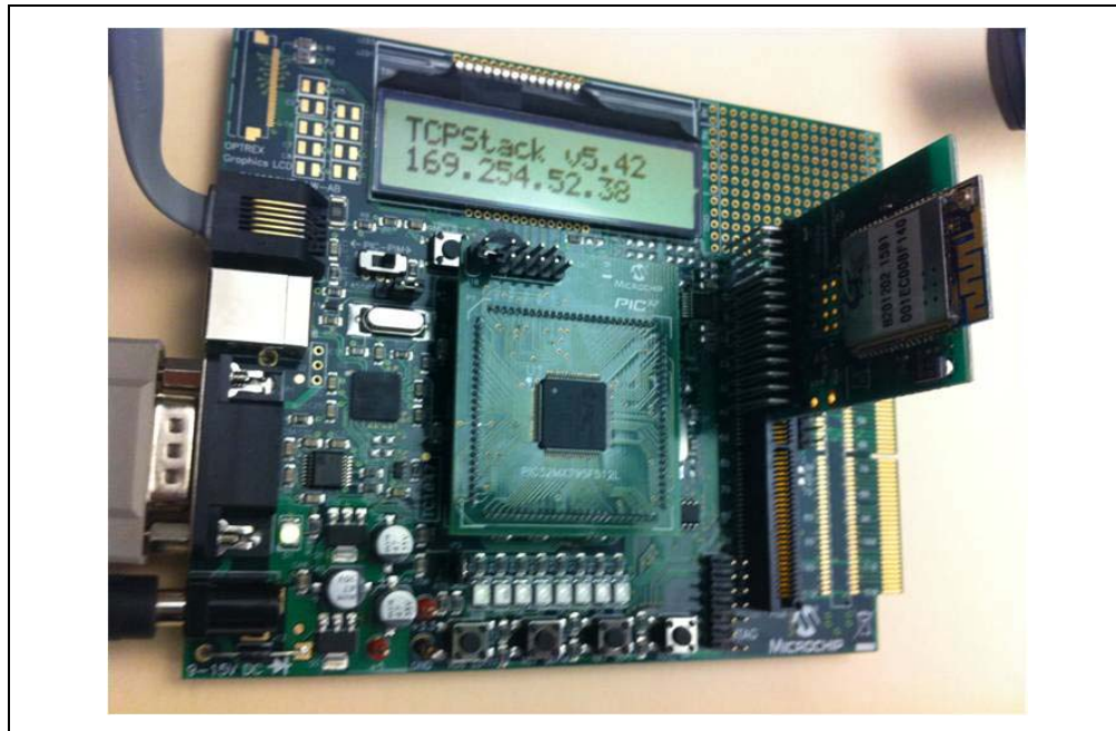
FIGURE 4-32: TCP/IP – DEMO APPLICATION: LEDS AND LCD ON DEVELOPMENT BOARD
