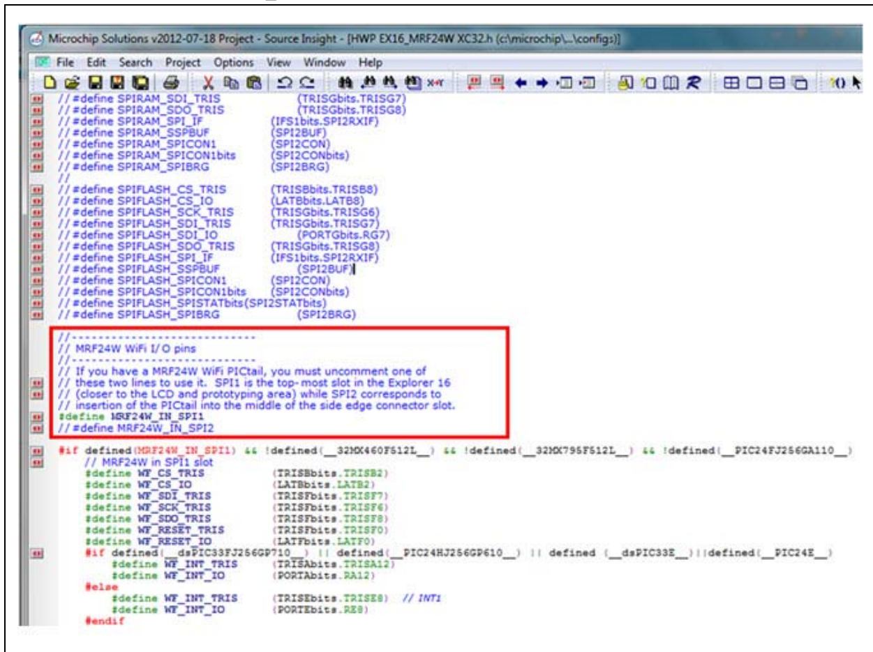
FIGURE 4-3: HWP EX16_MRF24W_XC32.H SPI OPTIONS
