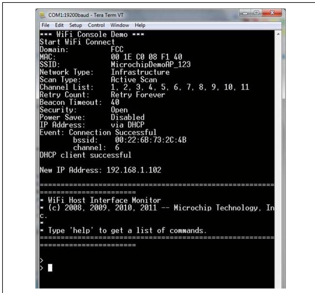
FIGURE 4-57: HYPERTERMINAL WINDOW READY
