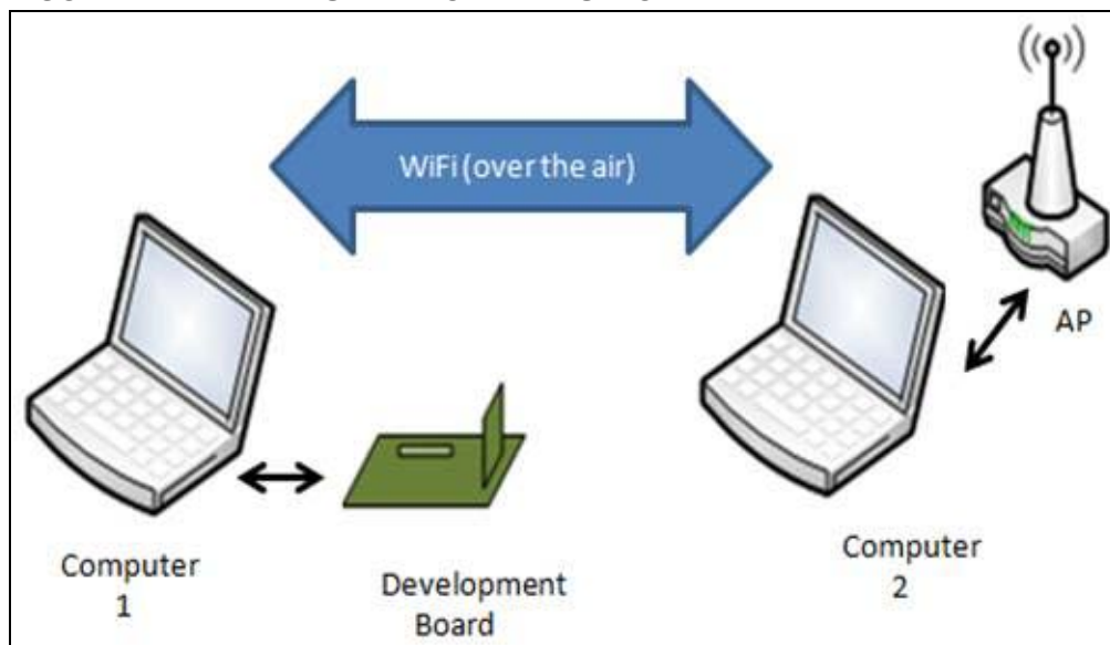
FIGURE 4-42: WPS ENVIRONMENT SETUP
