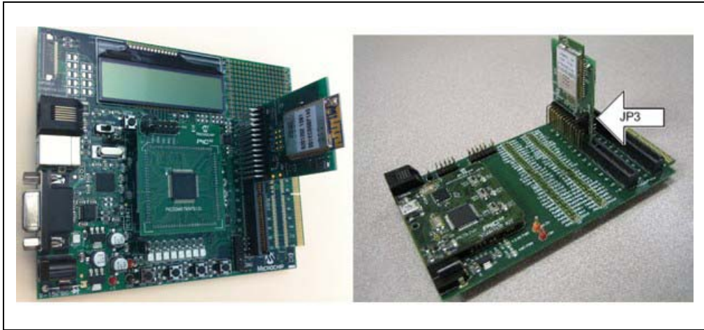
FIGURE 2-3: EXPLORER 16 AND PIC32 STARTER KIT WITH MRF24WB0MA/B OR MRF24WG0MA/B WI-FI® PICTAIL™
