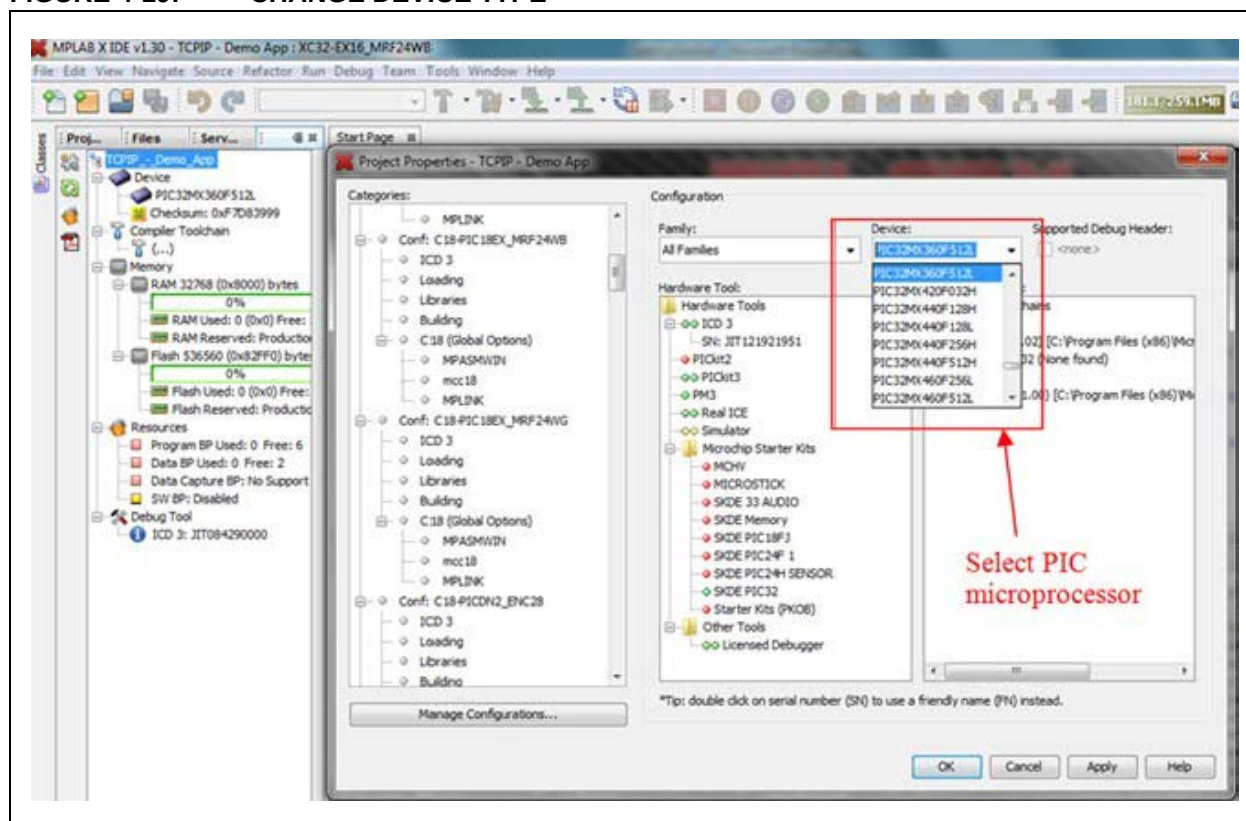
FIGURE 4-19: CHANGE DEVICE TYPE
