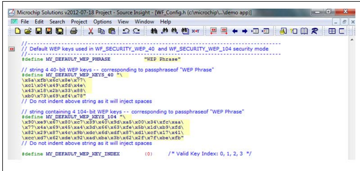
FIGURE 4-12: SOURCE CODE FOR WEP SECURITY SETUP
