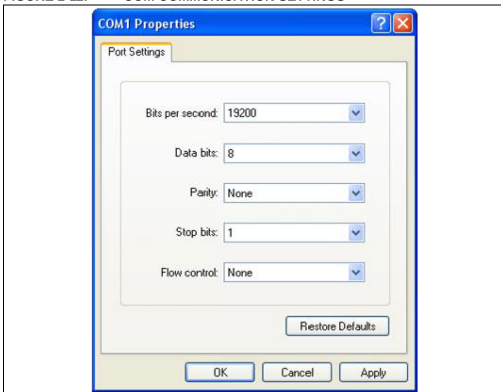
FIGURE 2-11: COM COMMUNICATION SETTINGS
