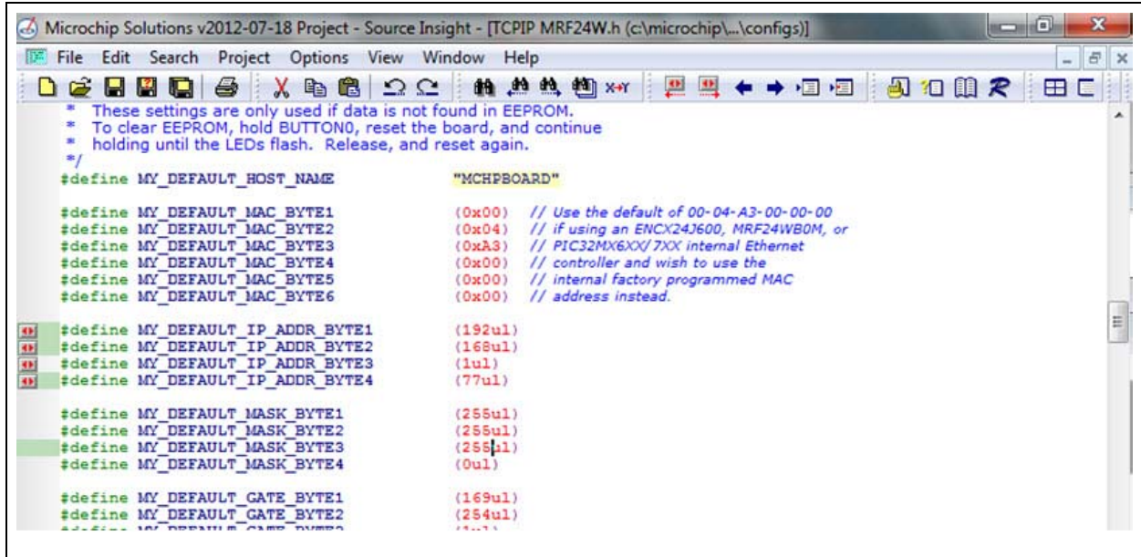
FIGURE 4-6: SETTING UP STATIC IP ADDRESS
