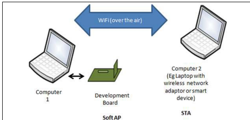
FIGURE 4-75: SOFTAP ENVIRONMENT SETUP
