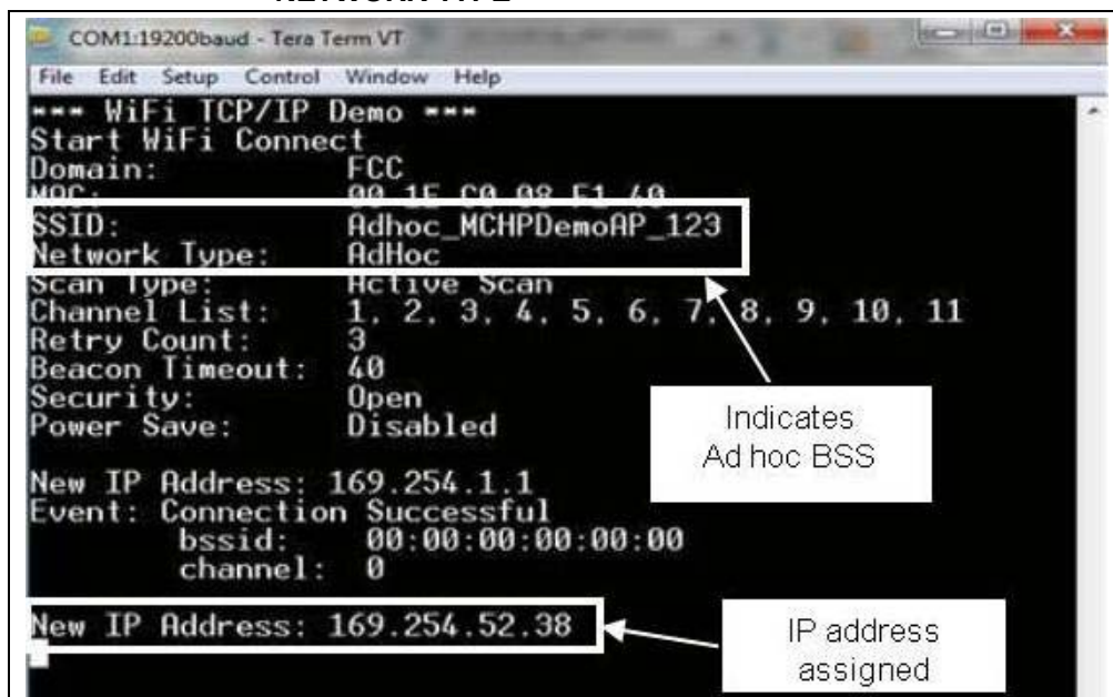
FIGURE 4-31: DEVELOPMENT BOARD SERIAL DISPLAY: AD HOC NETWORK TYPE
