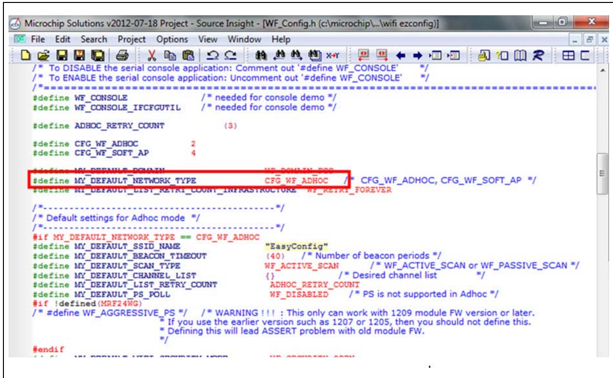
FIGURE 4-8: SOURCE CODE AD HOC SETTINGS
