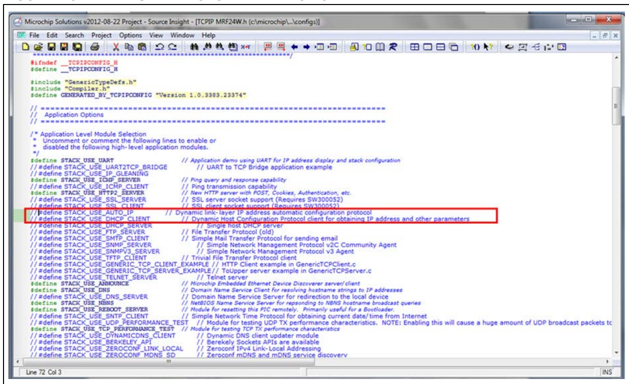
FIGURE 4-5: DISABLE AUTO IP AND DHCP CLIENT
