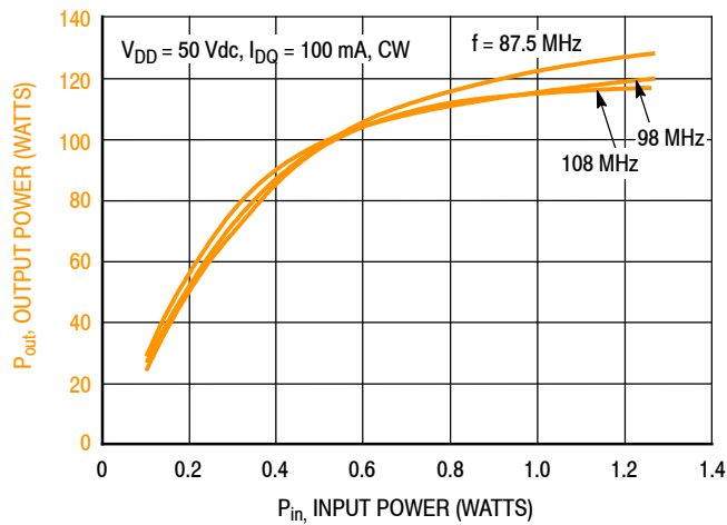
Figure 35. CW Output Power versus Input Power and Frequency
