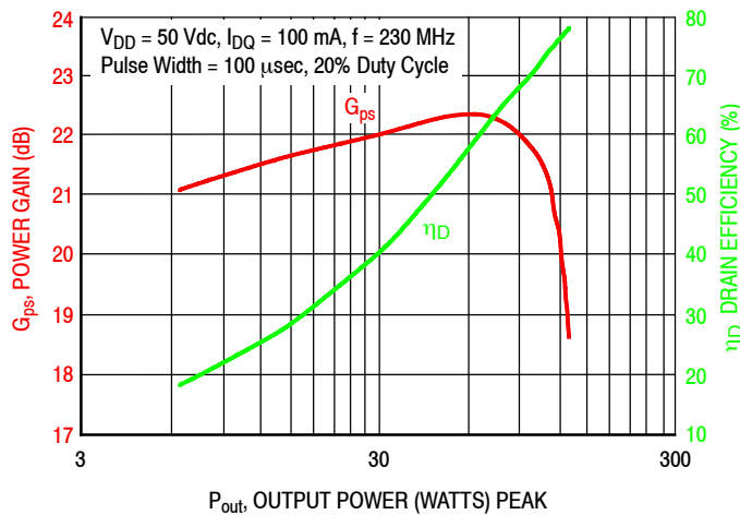
Figure 50. Power Gain and Drain Efficiency versus Output Power
