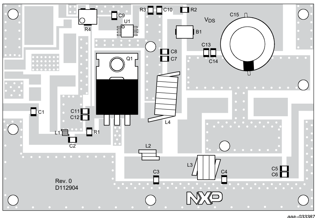
Figure 27. MRF101AN Reference Circuit Component Layout — 81.36 MHz
