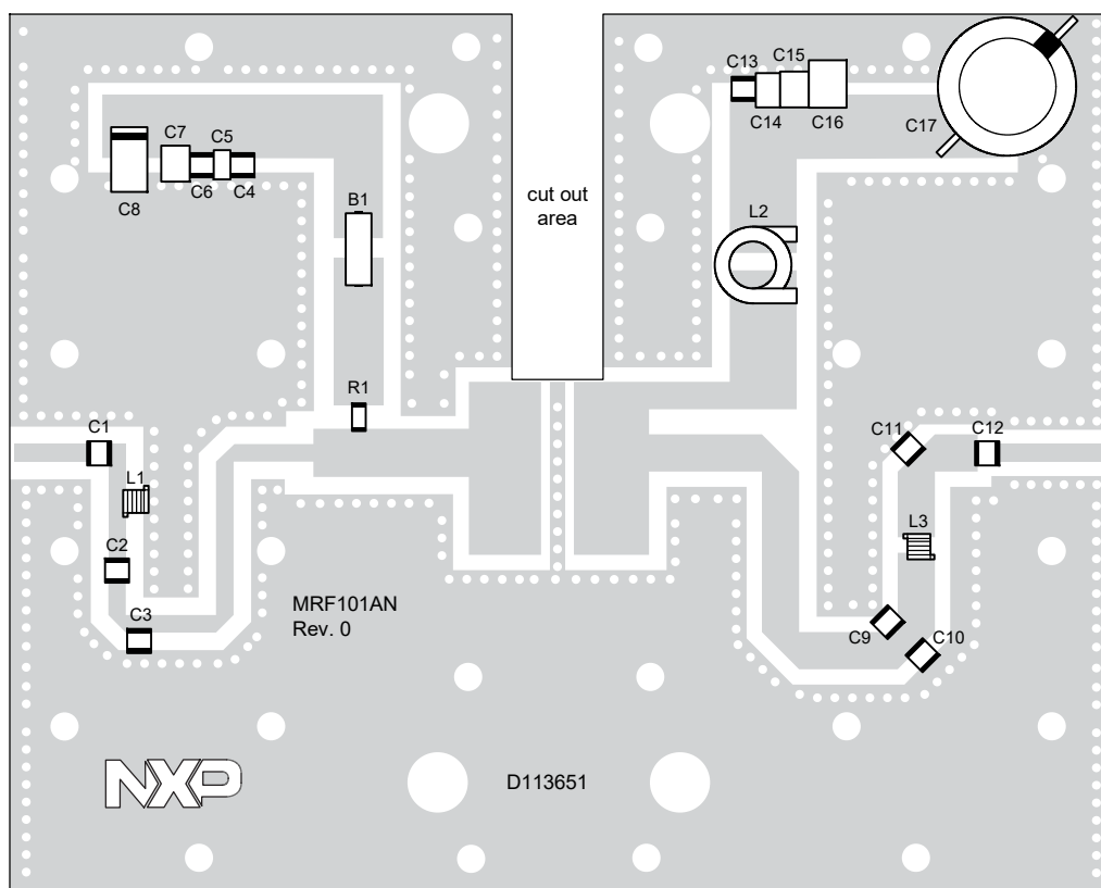
230 MHz FIXTURE (MRF101AN) — 4.0" x 5.0" (10.2 cm x 12.7 cm)
