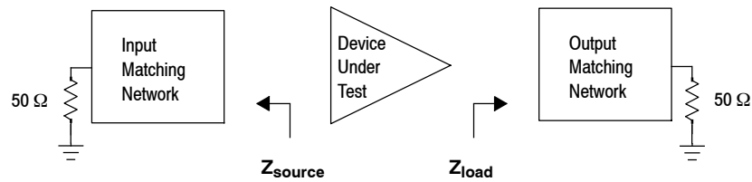
Figure 26. Series Equivalent Source and Load Impedance — 50 MHz
