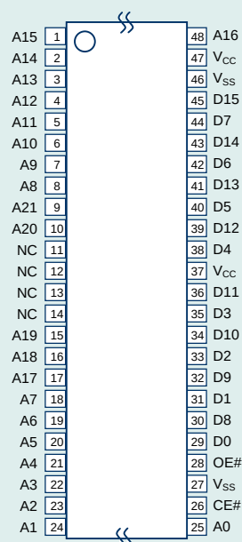
48TSOP(Type-I) TYPE I
