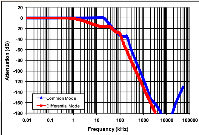
Figure 1: Typical Common Mode and Differential Mode Attenuation provided by the filter. Both input lines are connected to chassis ground through 50Ω resistors. The filter case is also connected to chassis ground.
