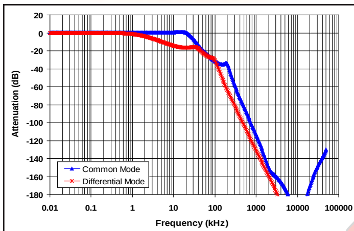
Figure 1: Typical Common Mode and Differential Mode Attenuation provided by the filter as a function of frequency. Both input lines are connected to chassis ground through 50ohm resistors. The filter case is also connected to chassis ground.
